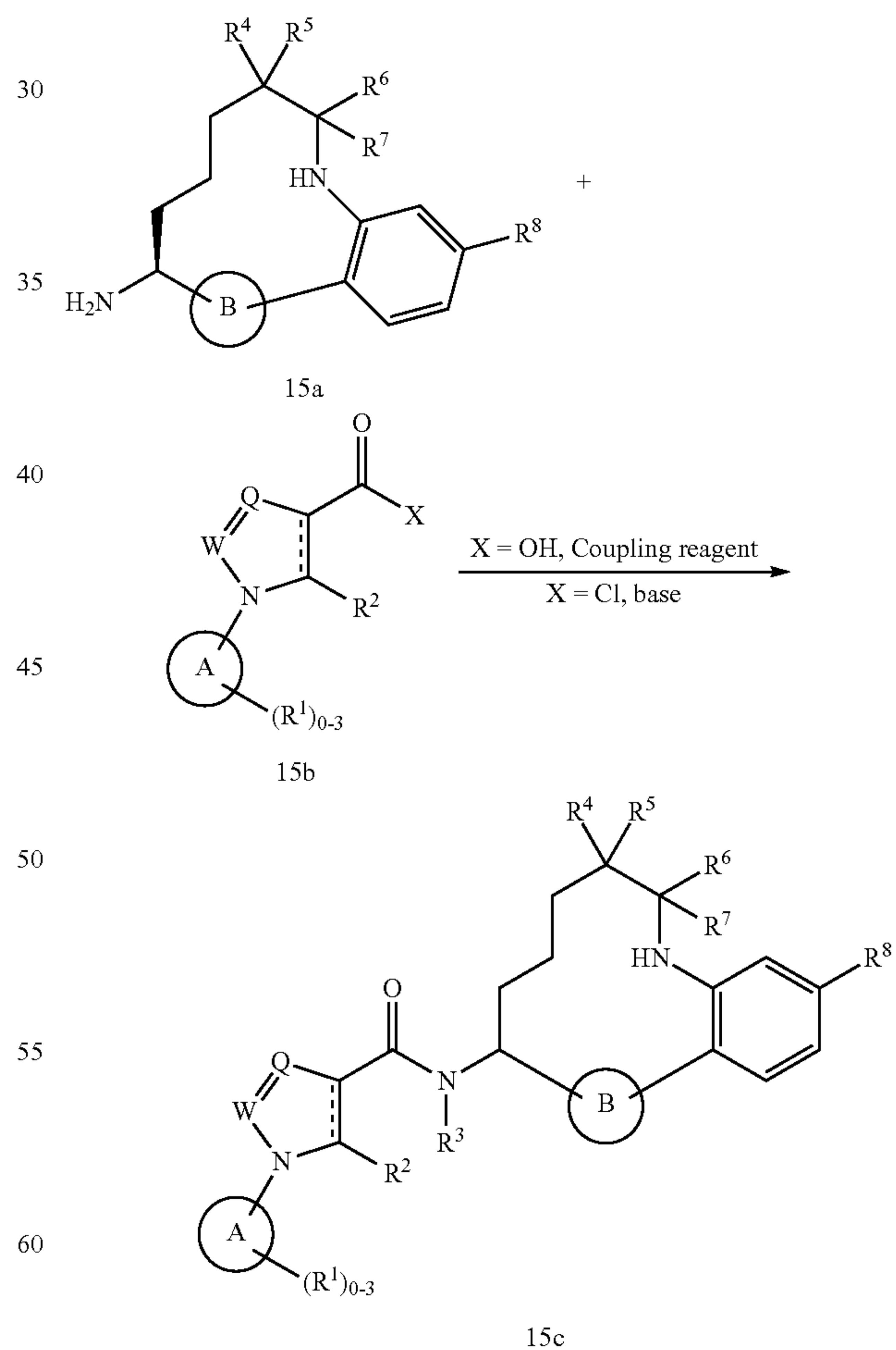
Scheme 15
