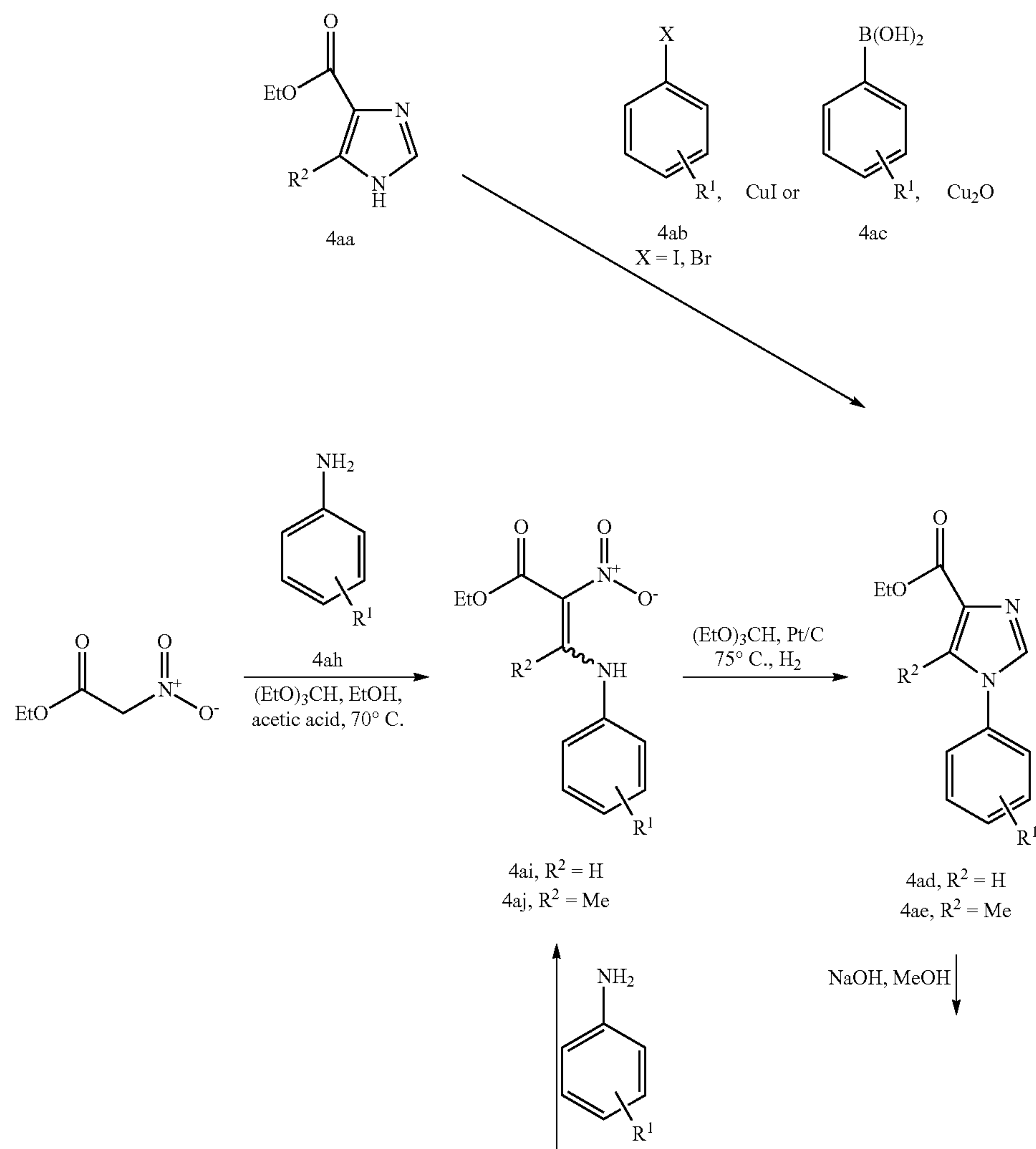
Scheme 4a
