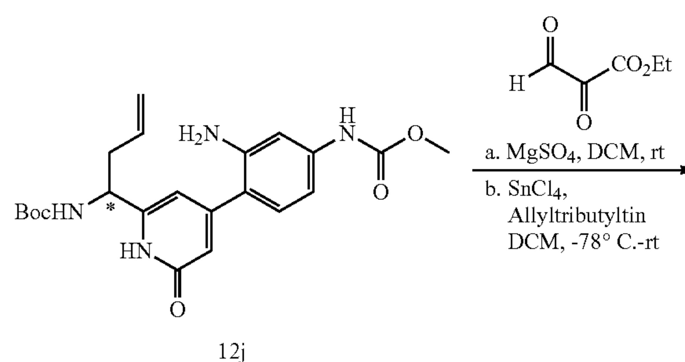
Scheme 13
