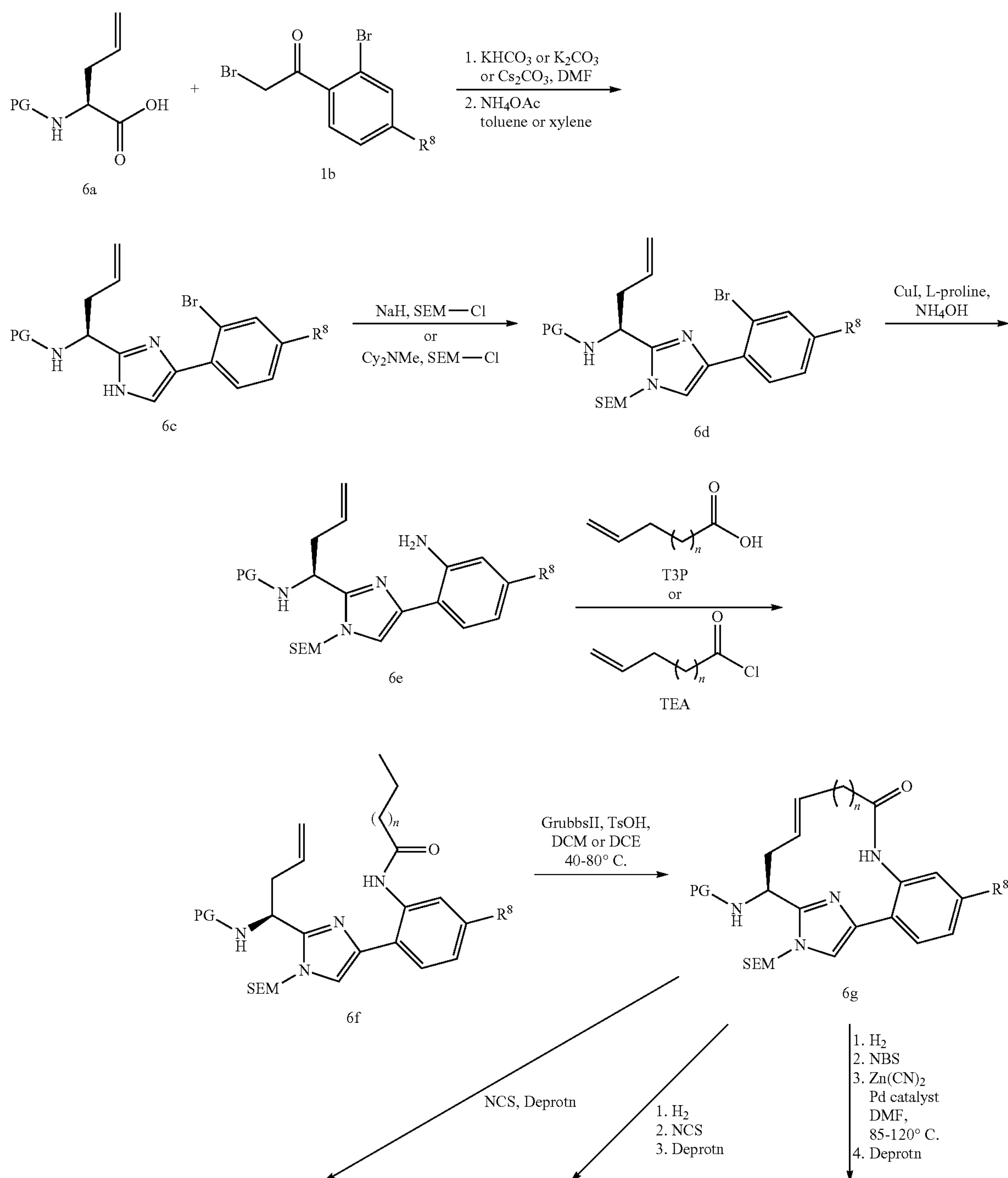
Scheme 6
