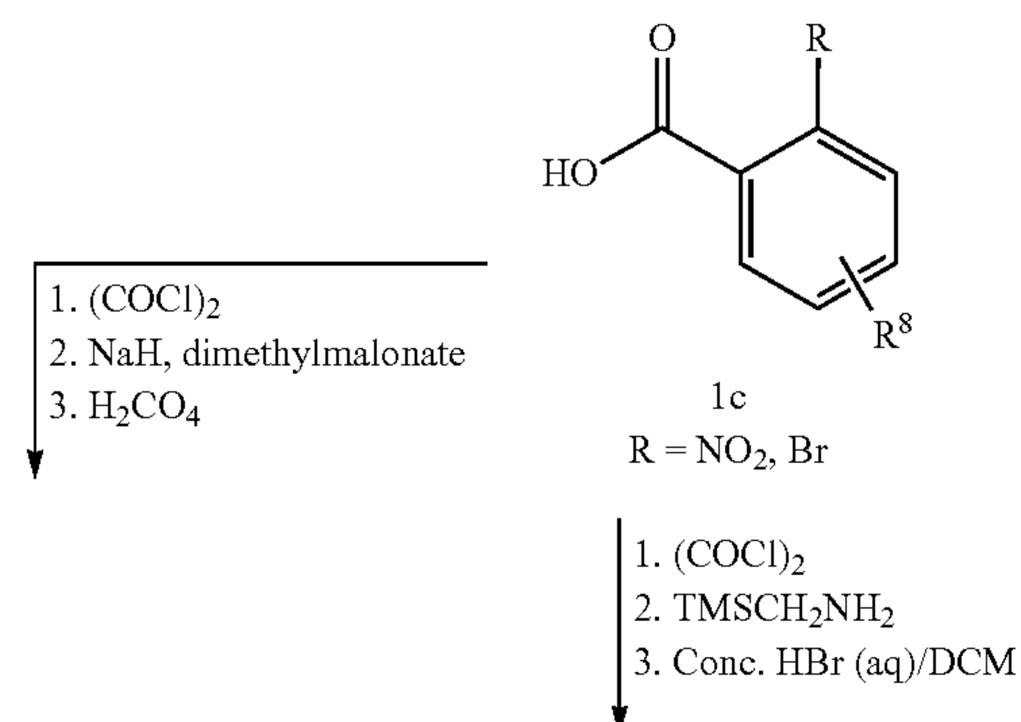
Scheme 1
