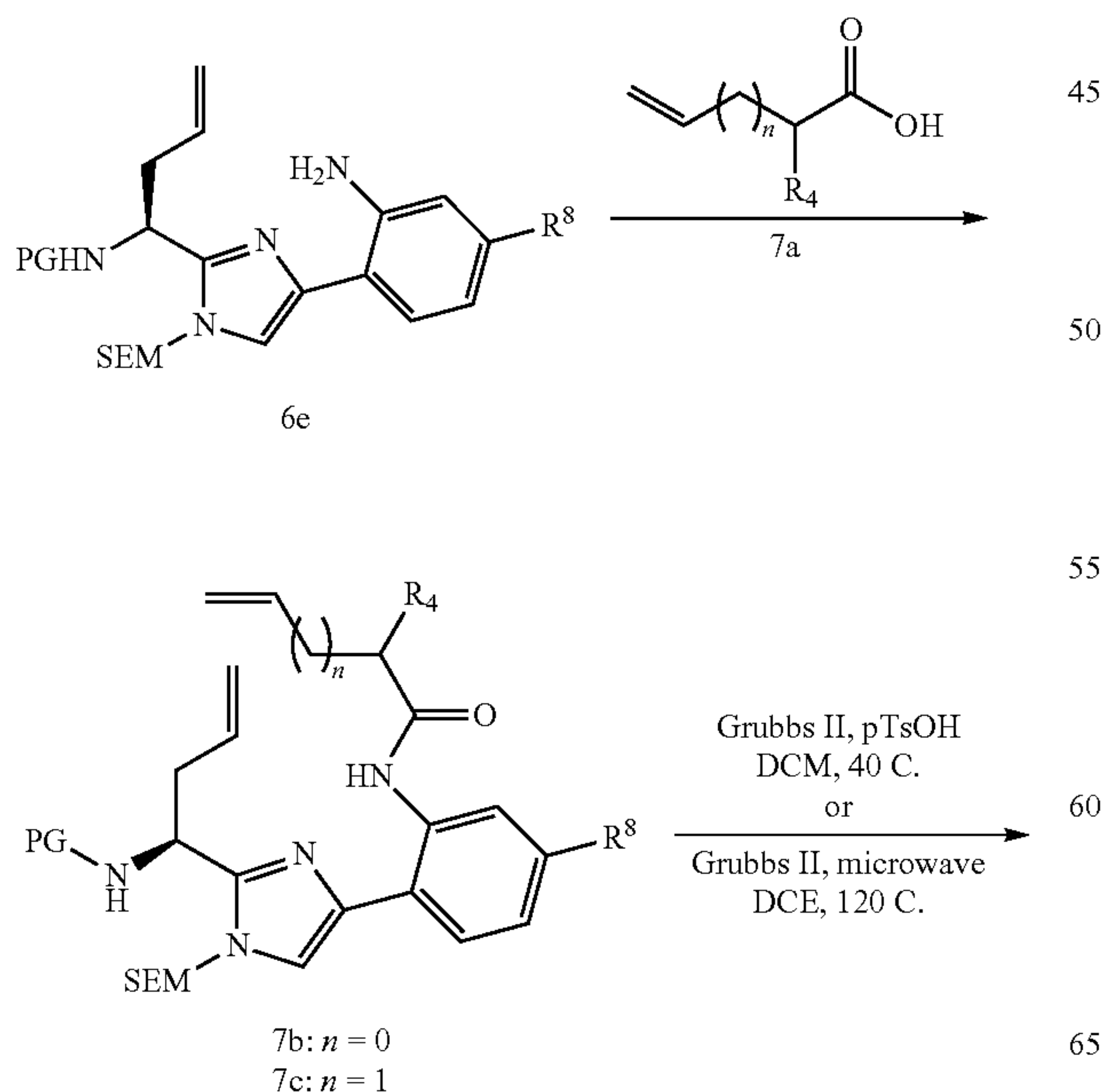
Scheme 7
