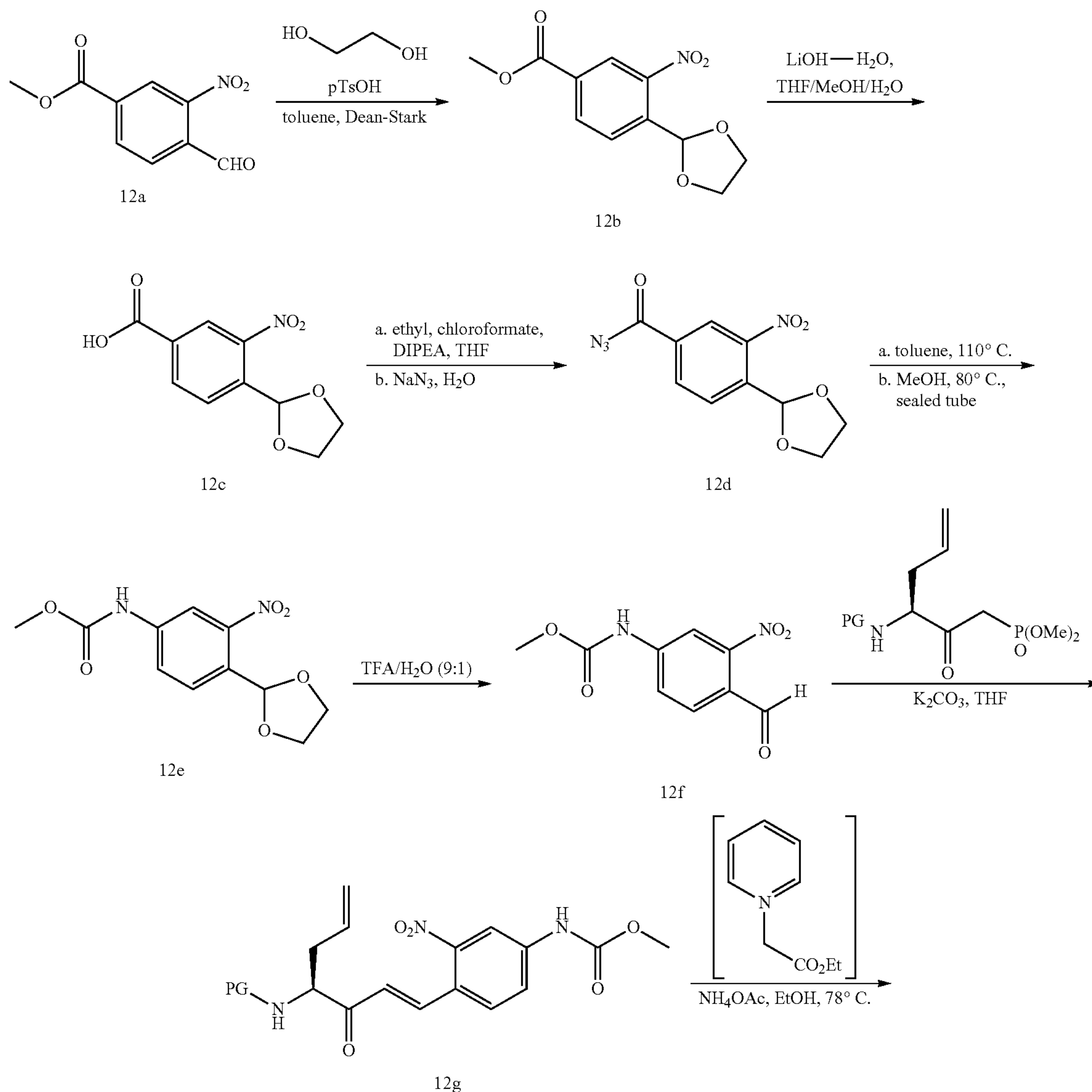
Scheme 12
