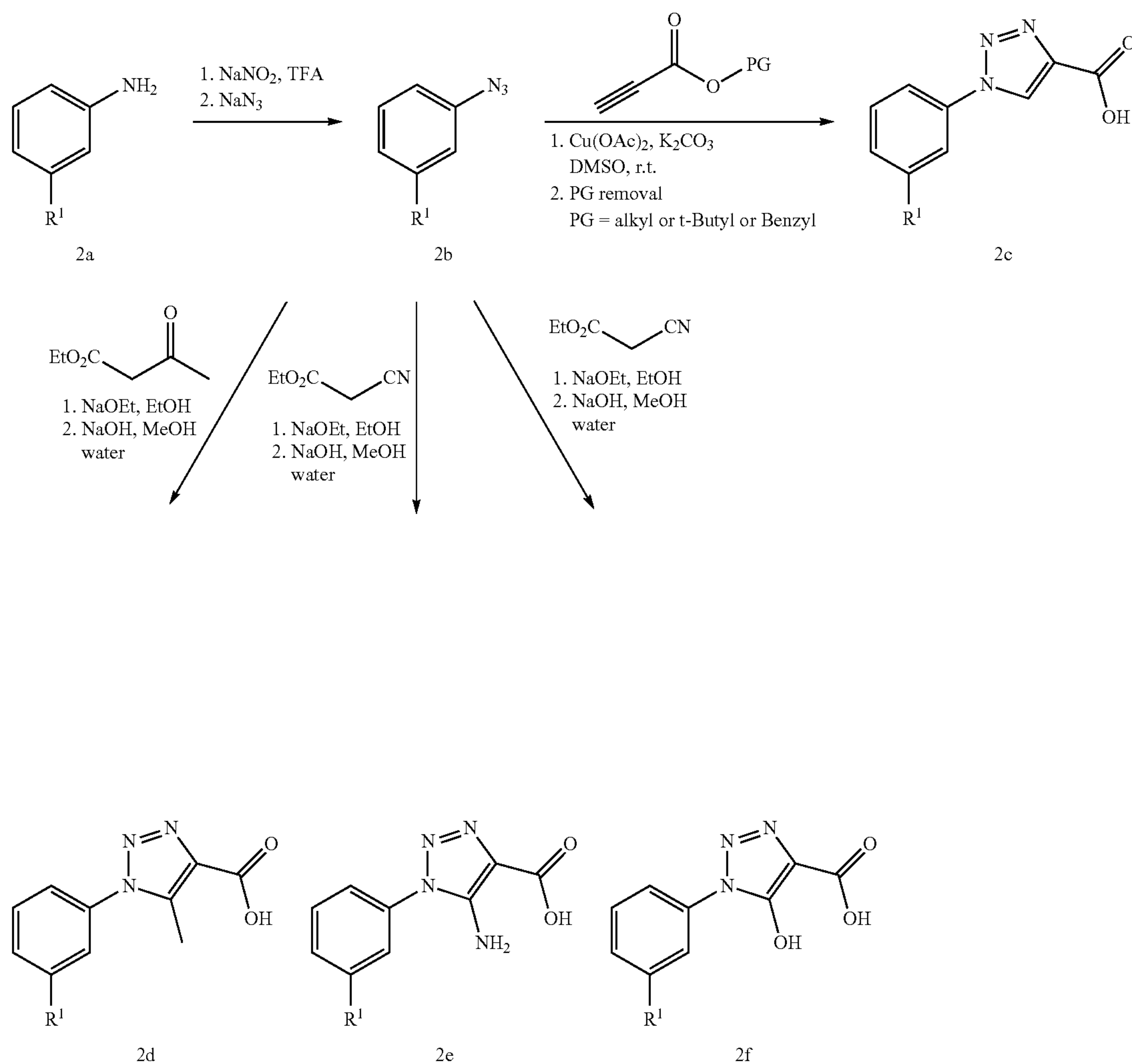
Scheme 2
