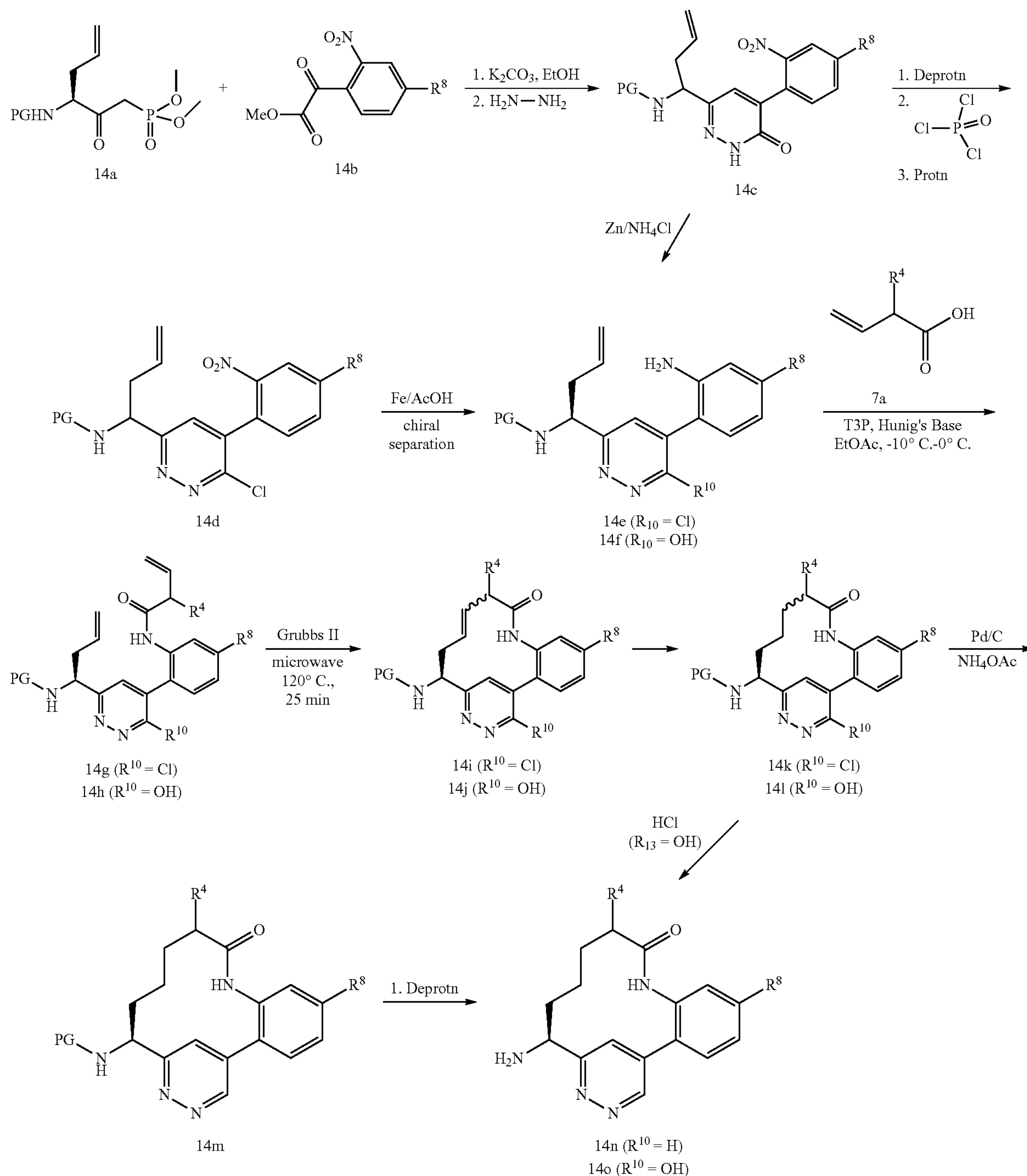
Scheme 14
