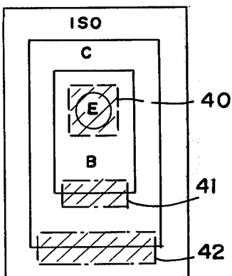
SUPER BETA NPN
