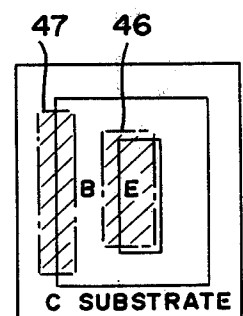
VERTICAL NPN
