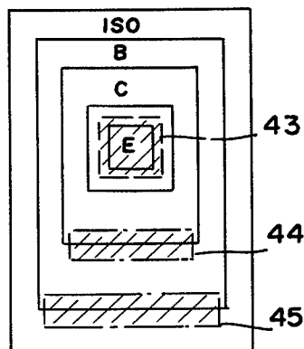
LATERAL NPN
