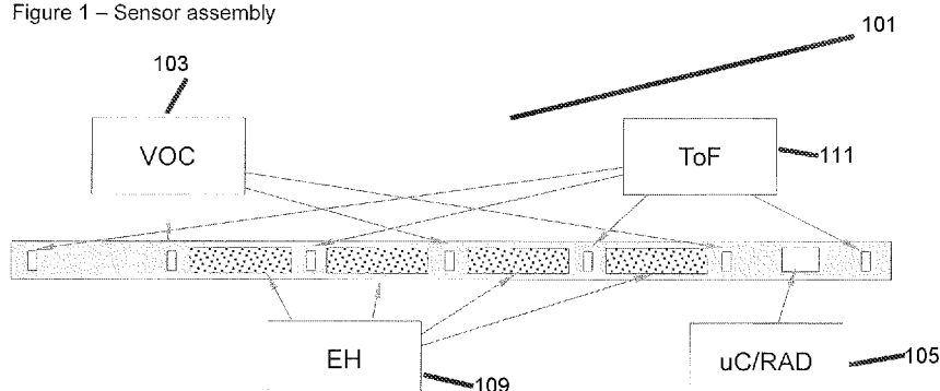
Figure 1 – Sensor assembly
