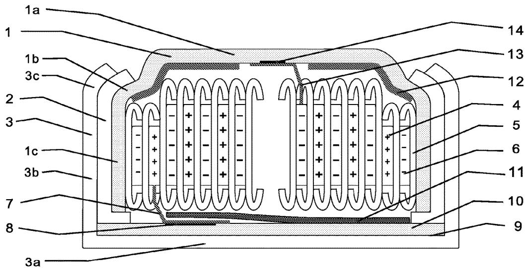
FIG. 6 (PRIOR ART)
