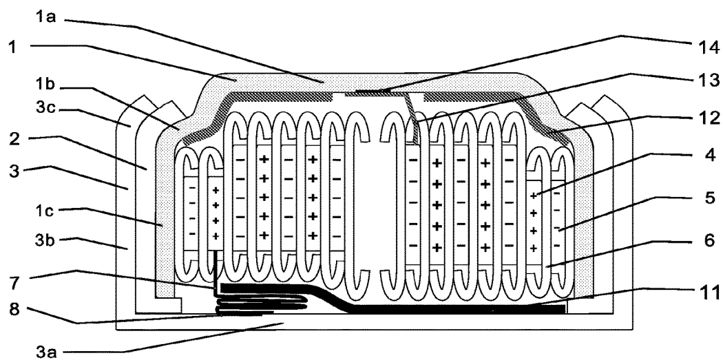
FIG. 7 (PRIOR ART)
