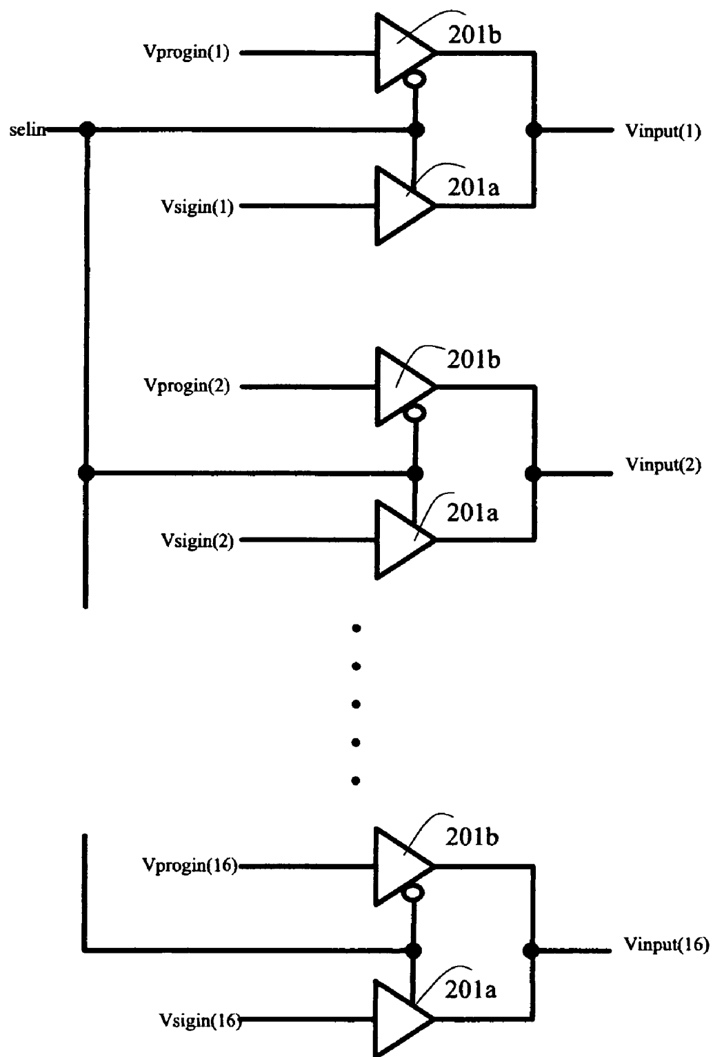
Fig.2 Input Selector Circuit
