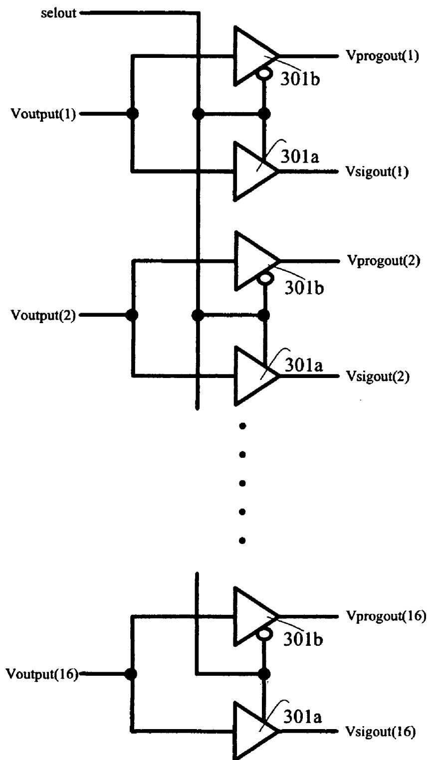
Fig.3 Output Selector Circuit
