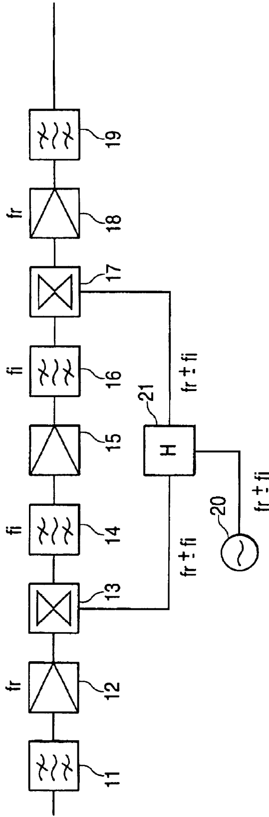
FIG. 4 (PRIOR ART)
