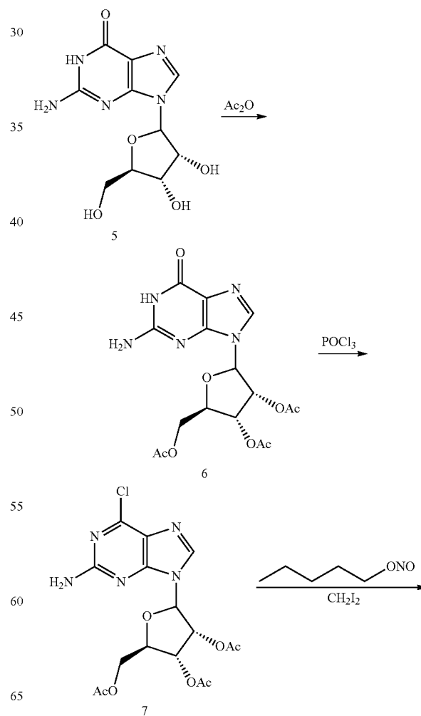
Scheme 3
