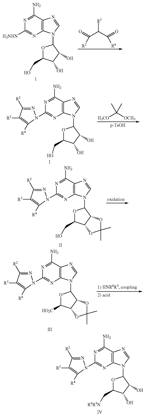
Scheme 1.
