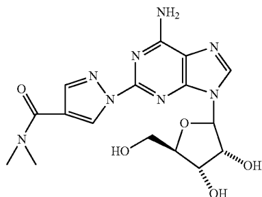
(1-{9-[(4S,2R,3R,5R)-3,4-dihydroxy-5-(hydroxymethyl)oxolan-2-yl]-6-aminopurin-2-yl}pyrazol-4-yl)-N,N-dimethylcarboxamide (18)
