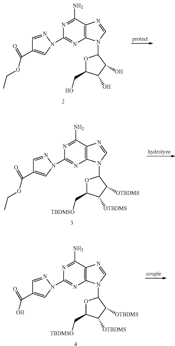
Scheme 2.
