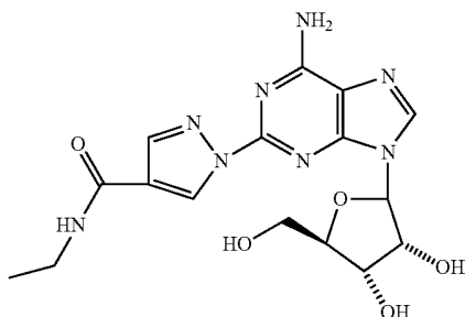
(1-{9-[(4S,2R,3R,5R)-3,4-dihydroxy-5-(hydroxymethyl)oxolan-2-yl]-6-aminopurin-2-yl}pyrazol-4-yl)-N-ethylcarboxamide (19)
