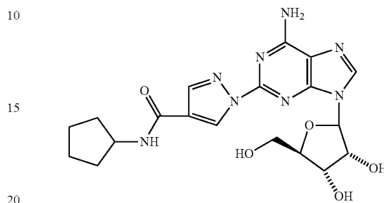
(1-{9-[(4S,2R,3R,5R)-3,4-dihydroxy-5-(hydroxymethyl)oxolan-2-yl]-6-aminopurin-2-yl}pyrazol-4-yl)-N-(cyclopentylmethyl)carboxamide (21)
