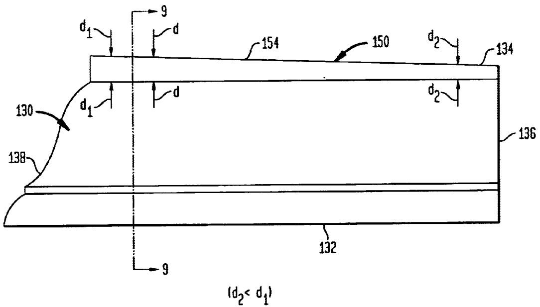
FIG. 8B (EXAGGERATED)
