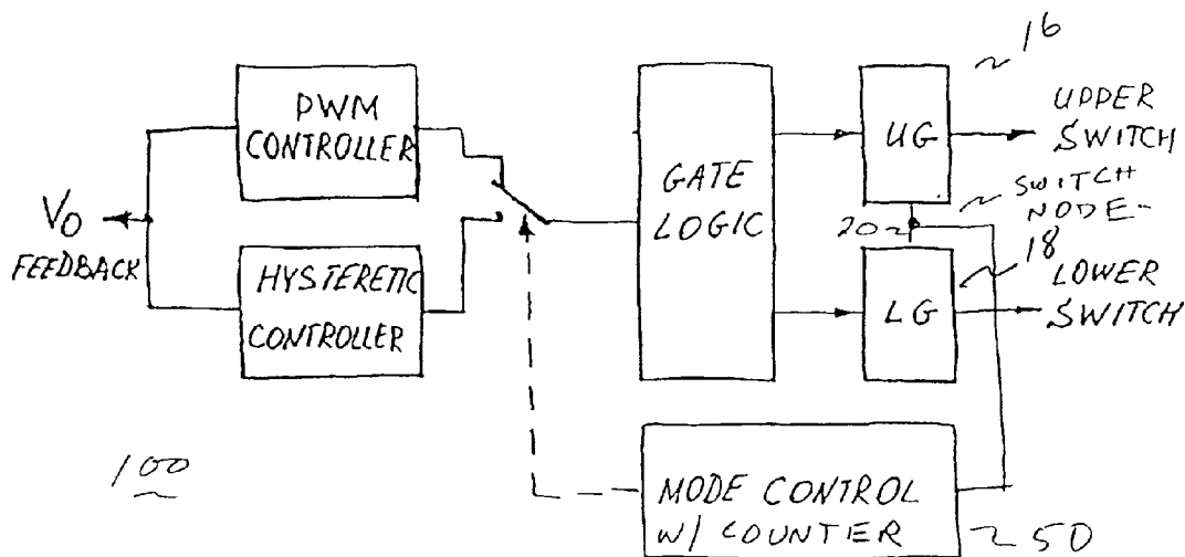
Fig. 4 Integrated controller
