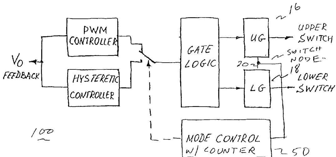
Integrated controller
