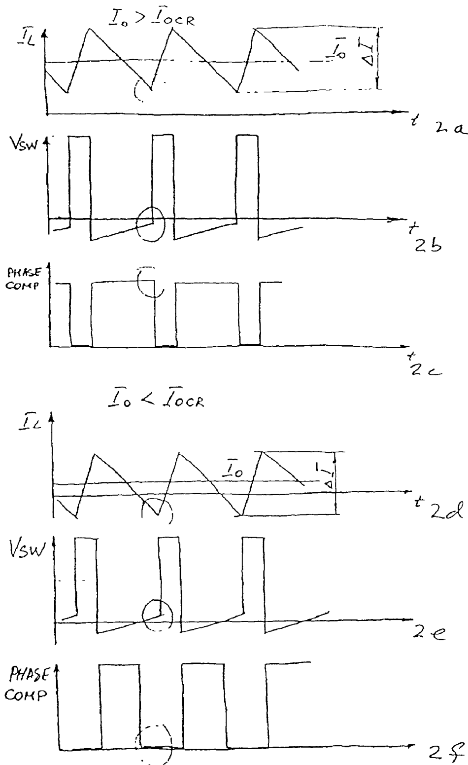
Fig. 2. Waveforms at different modes of operation
