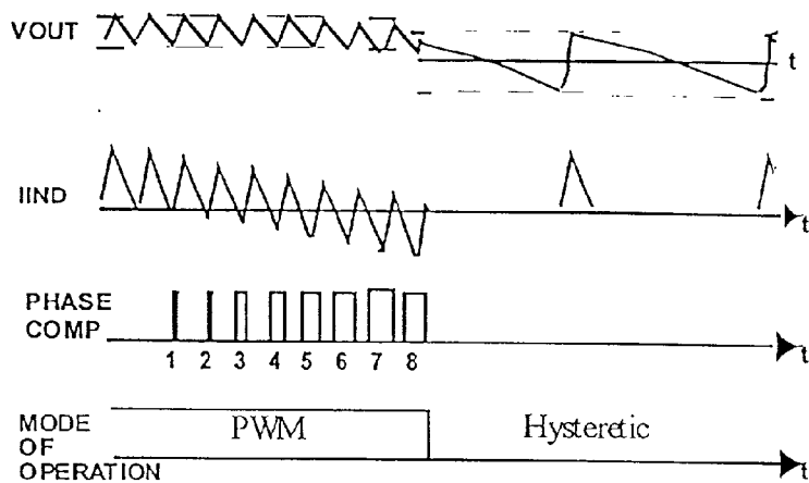
Fig. 3. Transition from PWM mode to hysteretic.
