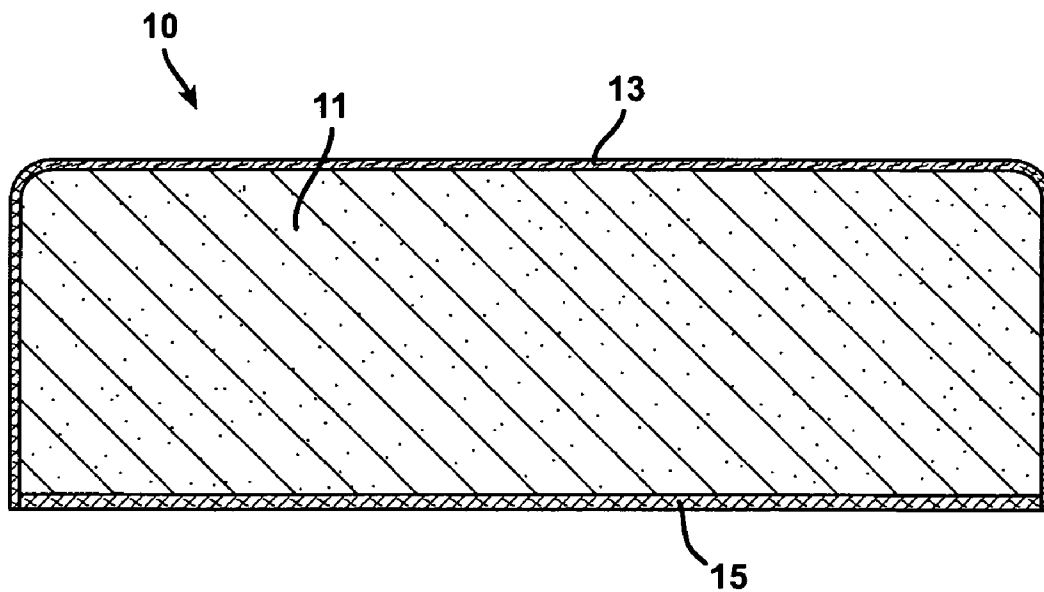
FIG. 2 PRIOR ART
