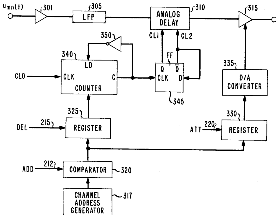
FIG. 3 CHANNEL CCT
