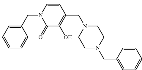
1-Benzyl-3-hydroxy-4-(4-benzylpiperazin-1-ylmethyl)pyridin-2(1H)-one
