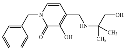
1-Benzyl-3-hydroxy-4-[(1-hydroxy-2-methylpropan-2-ylamino)methyl]pyridin-2(1H)-one
