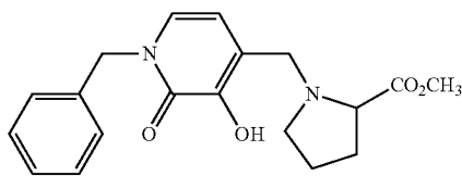
Methyl 1-[(1-benzyl-3-hydroxy-2-oxo-1,2-dihydropyridin-4-yl)methyl]pyrrolidine-2-carboxylate
