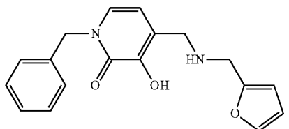
1-Benzyl-3-hydroxy-4-[[furan-2-ylmethyl]amino]methyl]pyridin-2(1H)-one
