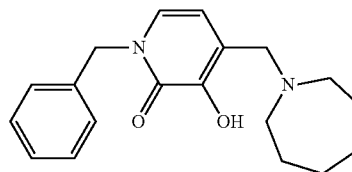
1-Benzyl-3-hydroxy-4-azepan-1-ylmethylpyridin-2(1H)-one
