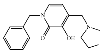
1-Benzyl-3-hydroxy-4-(thiazolidin-3-ylmethyl)pyridin-2(1H)-one
