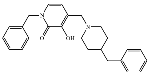
1-Benzyl-3-hydroxy-4-(4-benzylpiperidin-1-ylmethyl)pyridin-2(1H)-one
