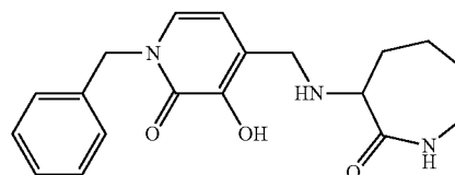
3-[(1-Benzyl-3-hydroxy-2-oxo-1,2-dihydropyridin-4-yl)methylamino]azepan-2-one
