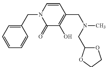
1-Benzyl-3-hydroxy-4-[(1,3]-dioxolan-2-ylmethylmethylamino)methyl]pyridin-2(1H)-one
