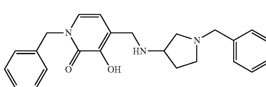
1-Benzyl-3-hydroxy-4-[(1-benzylpyrrolidin-3-ylamino)methyl]pyridin-2(1H)-one
