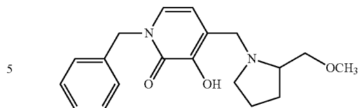
1-Benzyl-3-hydroxy-4-[[2-(methoxymethyl)pyrrolidin-1-yl]methyl]pyridin-2(1H)-one
