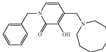
1-Benzyl-3-hydroxy-4-(azocan-1-ylmethyl)pyridin-2(1H)-one
