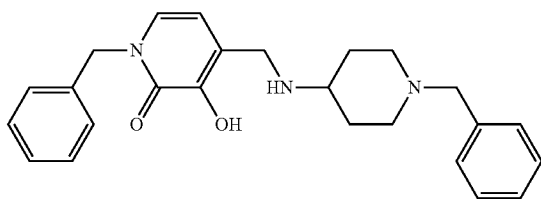
1-Benzyl-3-hydroxy-4-[(1-benzylpiperidin-4-ylamino)methyl]pyridin-2(1H)-one
