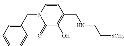
1-Benzyl-3-hydroxy-4-[[2-(methylthio)ethylamino]methyl]pyridin-2(1H)-one
