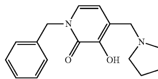
1-Benzyl-3-hydroxy-4-(pyrrolidin-1-ylmethyl)pyridin-2(1H)-one
