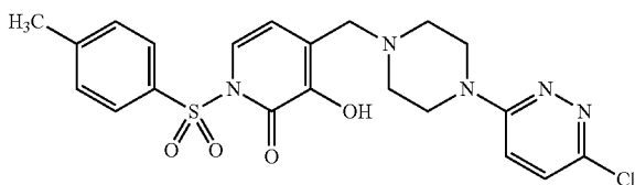
1-(4'-Methylbenzenesulfonyl)-3-hydroxy-4-[4-(6-chloropyridazin-3-yl)piperazin-1-ylmethyl]pyridin-2(1H)-one
