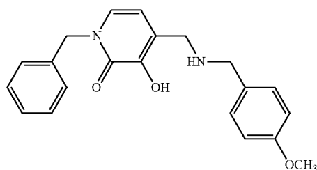
1-Benzyl-3-hydroxy-4-[(4-methoxybenzylamino)methyl]pyridin-2(1H)-one
