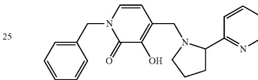
1-Benzyl-3-hydroxy-4-[[2-(pyridin-2-yl)pyrrolidin-1-yl]methyl]pyridin-2(1H)-one
