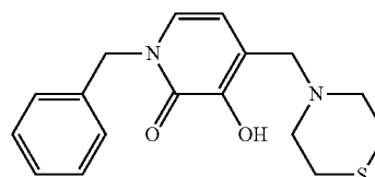
1-Benzyl-3-hydroxy-4-(thiomorpholin-4-ylmethyl)pyridin-2(1H)-one
