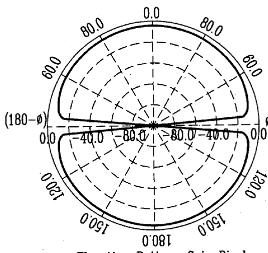
Elevation Pattern Gain Display (dBi)
