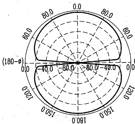
Elevation Pattern Gain Display (dBi)
