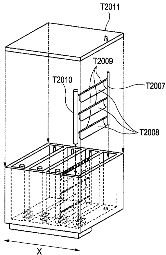
FIG. 17 PRIOR ART
