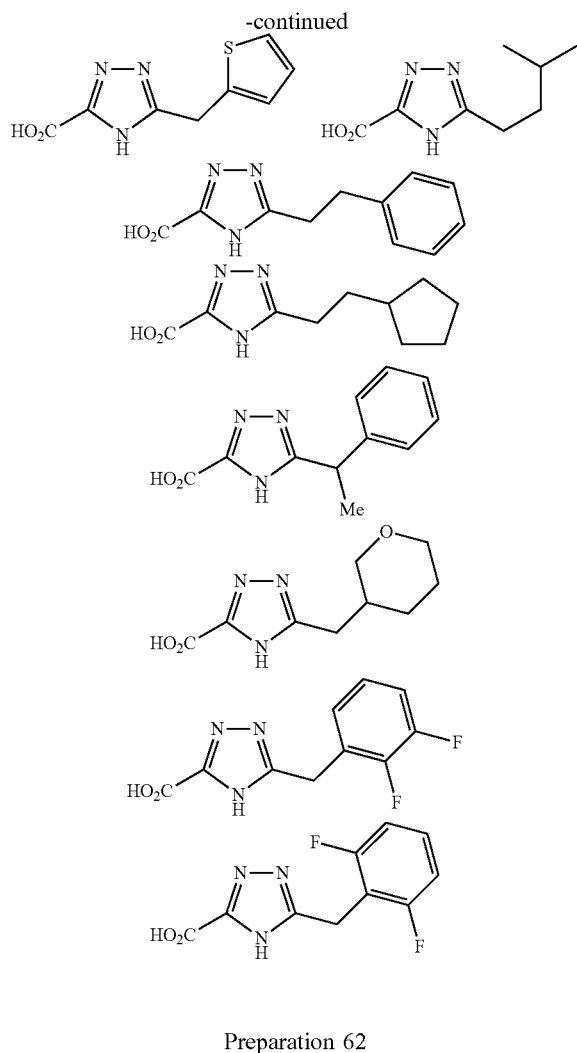
ethyl 1-(3-(3-fluorobenzyl)-1H-imidazol-4-yl)carboxylate [0402]
