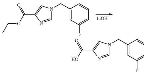
1-(3-(3-fluorobenzyl)-1H-imidazole-4-carboxylic acid [0405]
