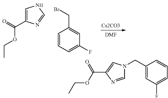
ethyl 1-(3-(3-fluorobenzyl)-1H-imidazol-4-yl)carboxylate [0402]
