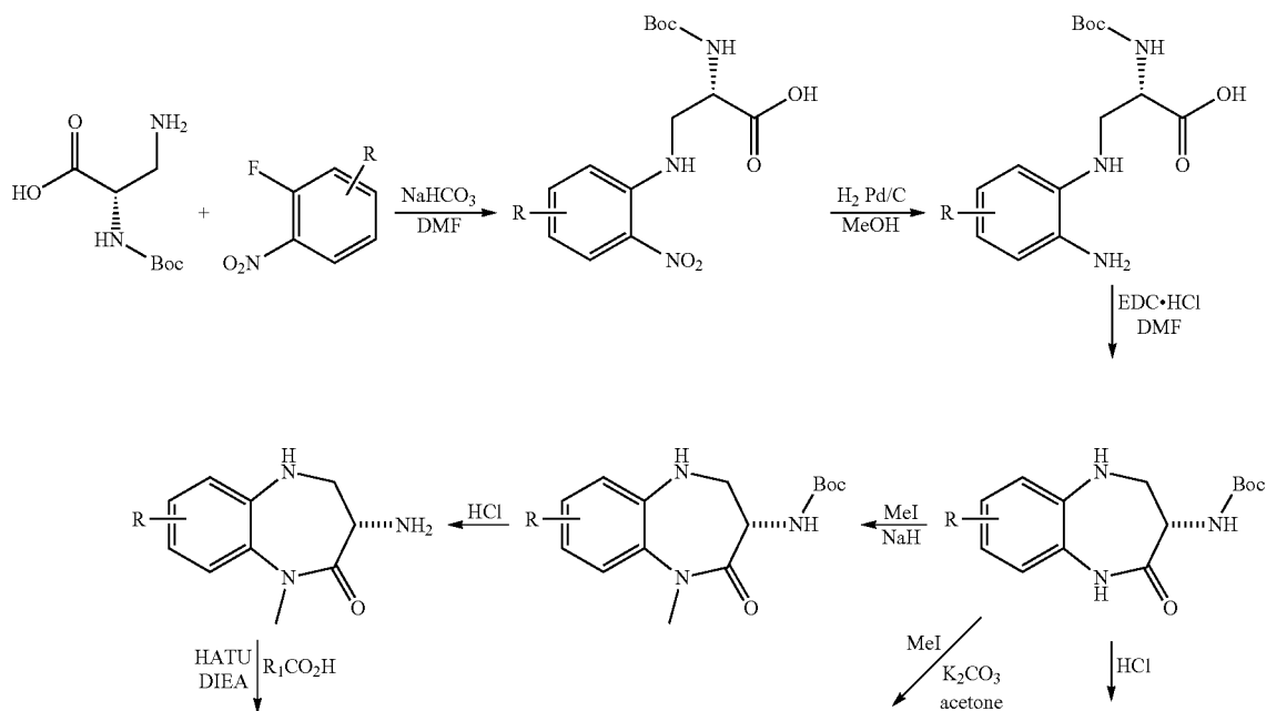
Scheme 3
