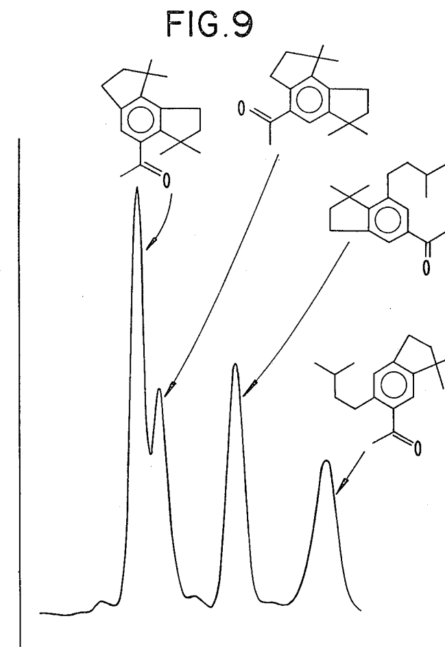
GLC PROFILE FOR EXAMPLE V
