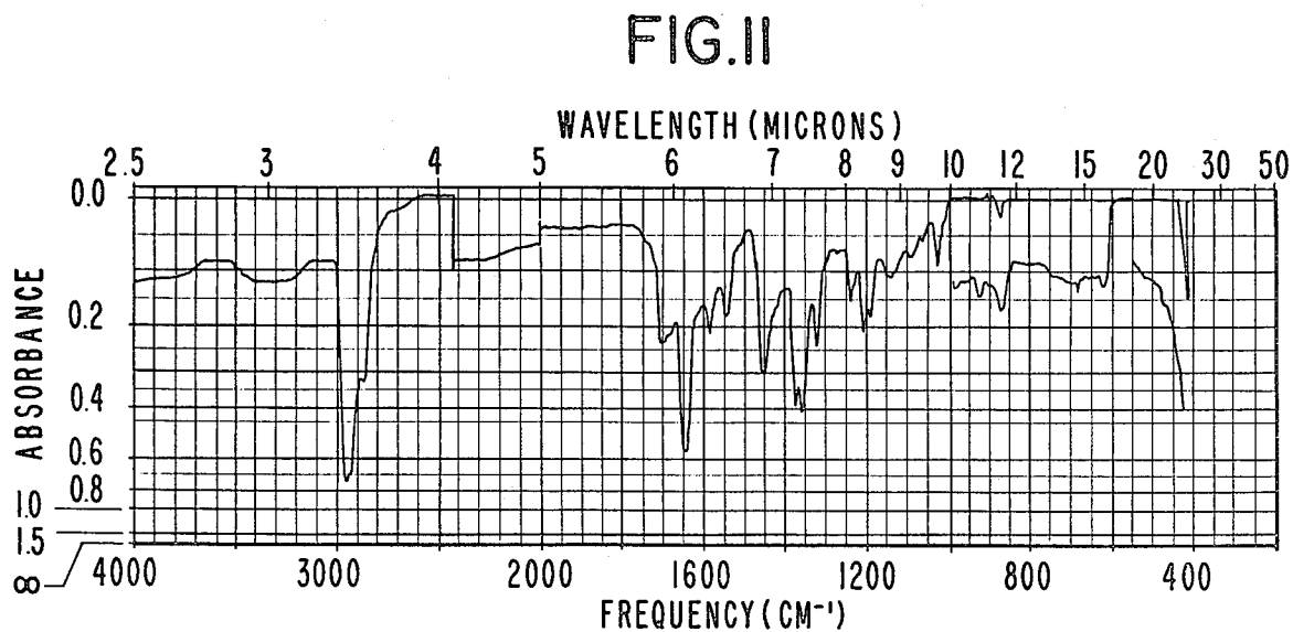
IR SPECTRUM FOR EXAMPLE V.
