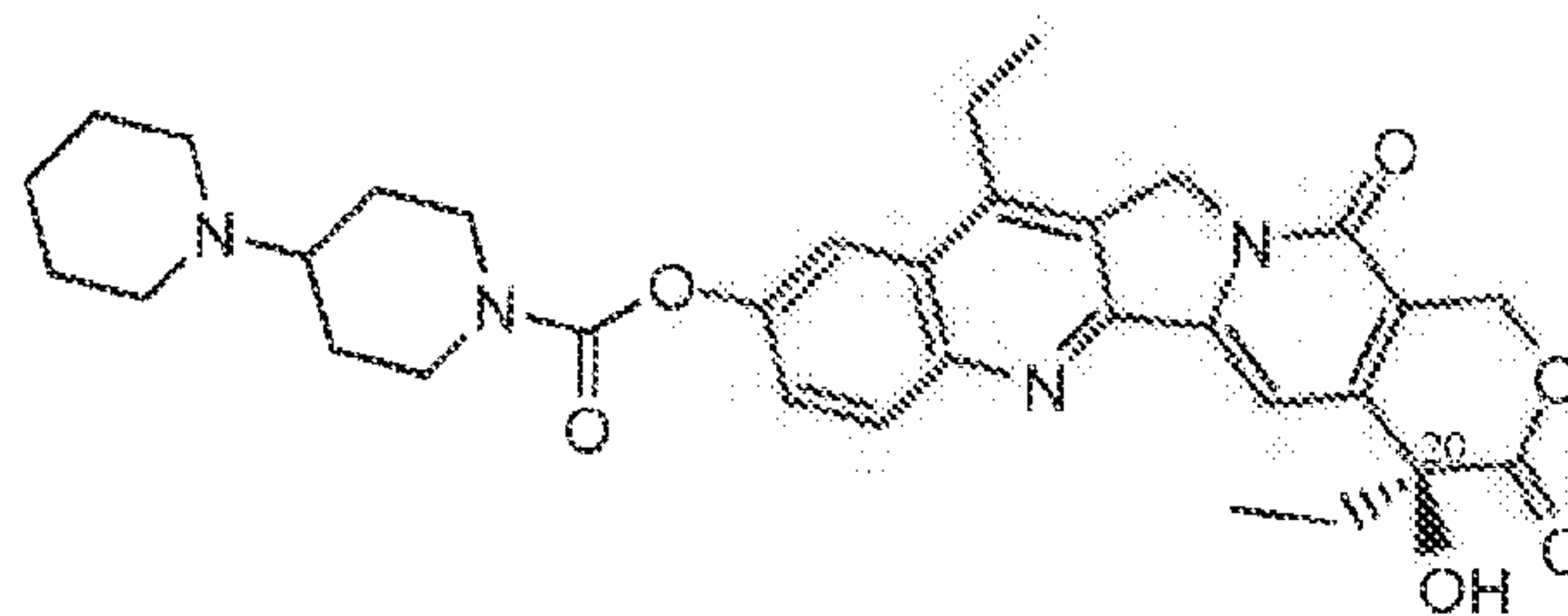
Irinotecan
