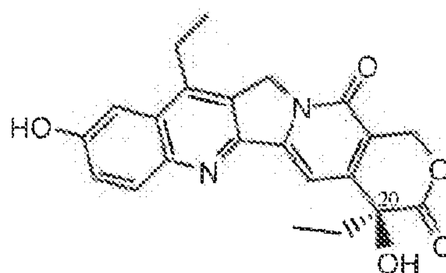
7-ethyl-10-hydroxy-camptothecin
