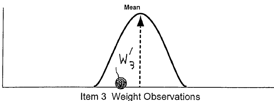
Figure 4c. Item 3 Weight Distribution and Shifted Weight Sample
