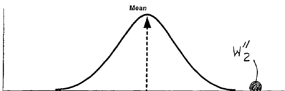
Item 2 Weight Observations
