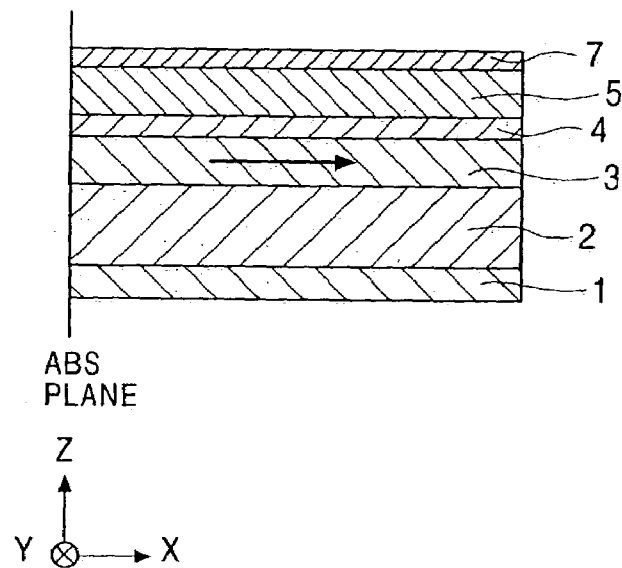
FIG. 29 PRIOR ART
