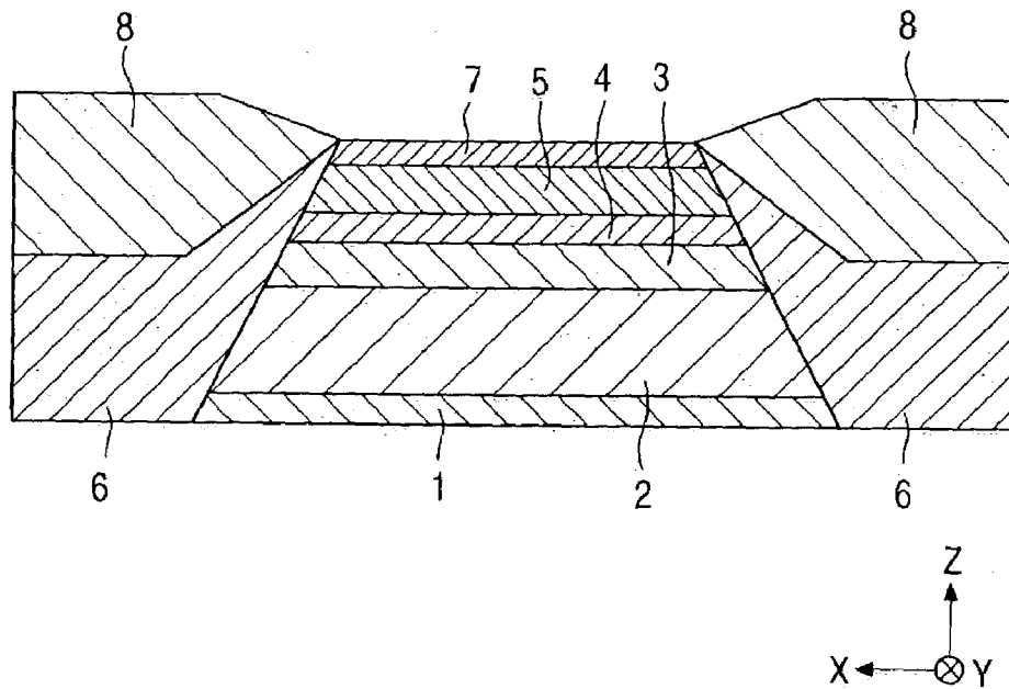
FIG. 28 PRIOR ART
