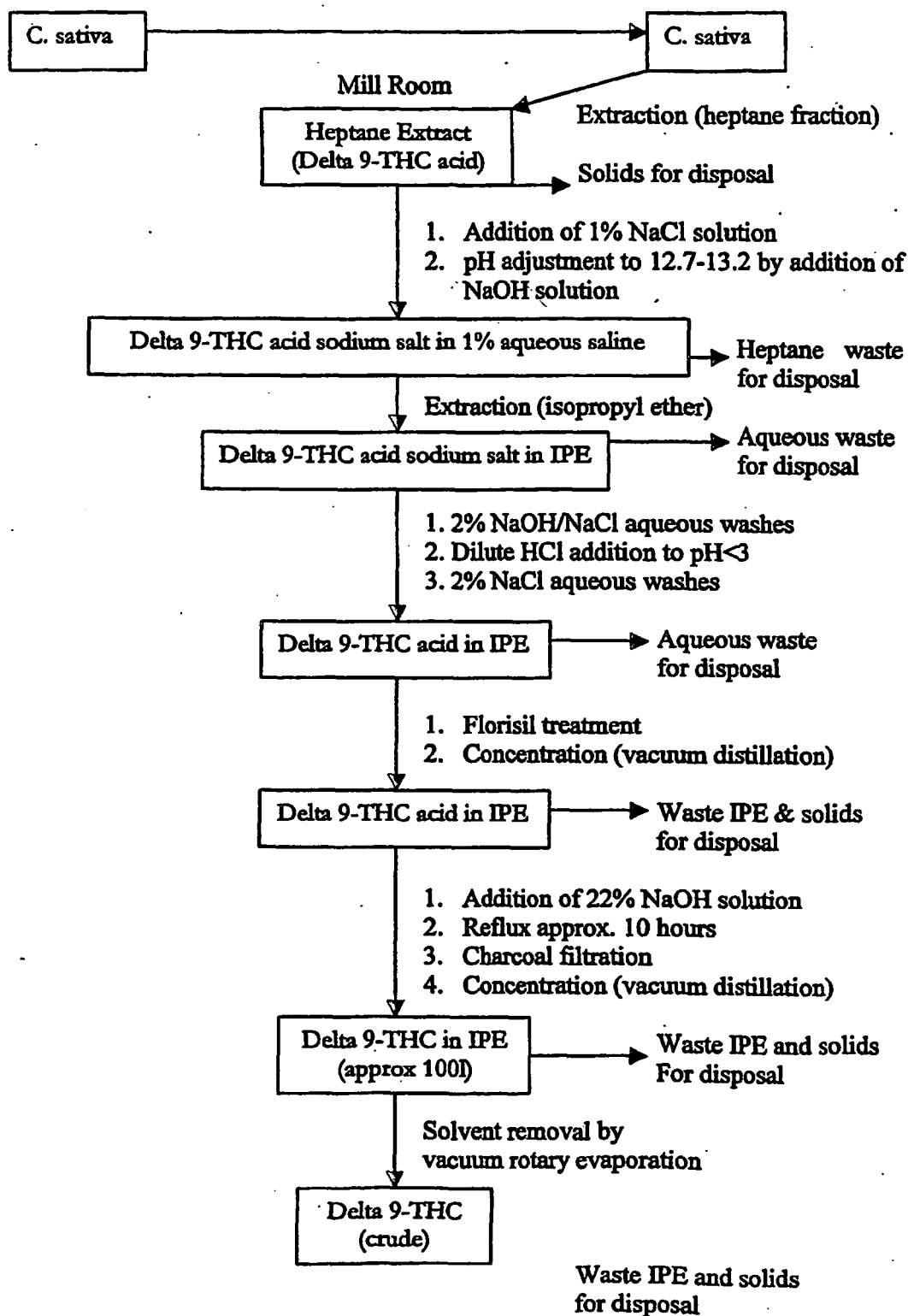
Figure 1 - Delta 9 THC Extraction
