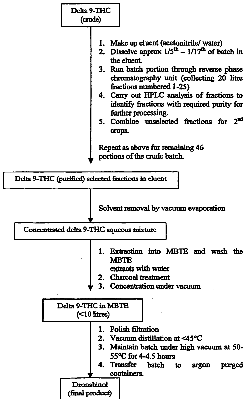
Figure 2 – Delta 9 THC Purification
