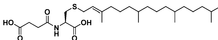
Compound N-48
