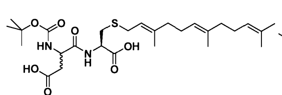
N-64;
