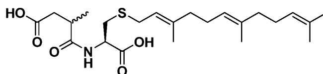
Compound N-21
