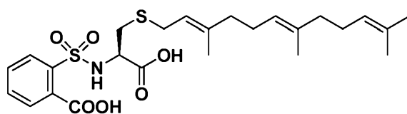
Compound N-81
