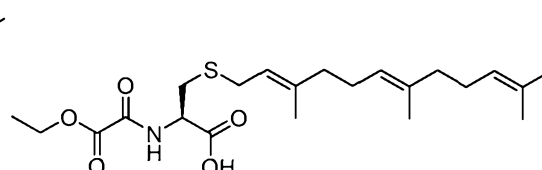
N-13;
