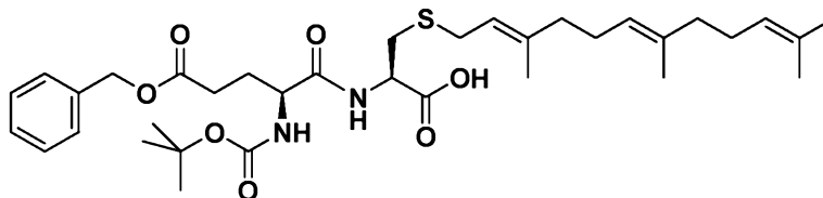
Compound N-63
