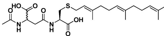
Compound N-32
