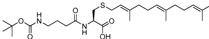
Compound N-7
