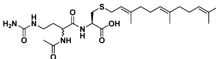
Compound N-77
