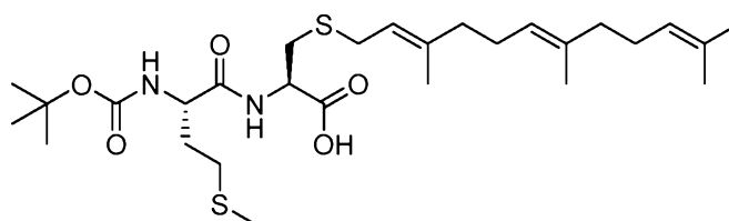
Compound N-57
