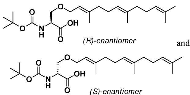
Compound N-54
