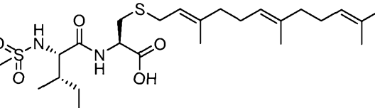
N-67;
