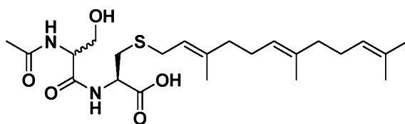
Compound N-23
