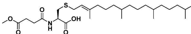
Compound N-53
