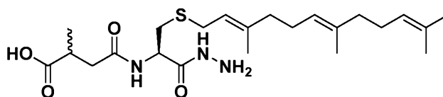
Compound N-34
