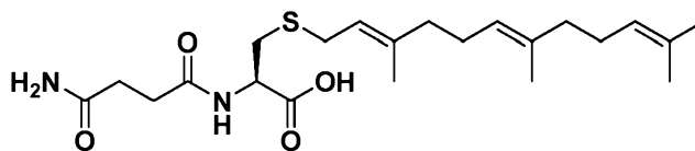
Compound N-26
