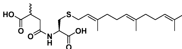
Compound N-22
