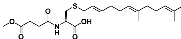
Compound N-17
