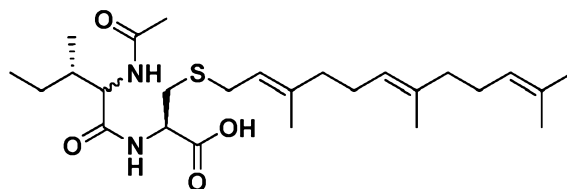
Compound N-62
