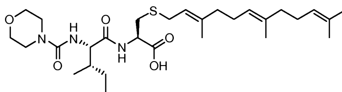
Compound N-70
