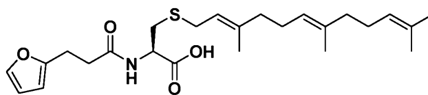
Compound N-96
