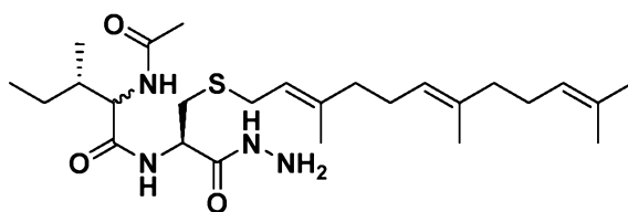
Compound N-72
