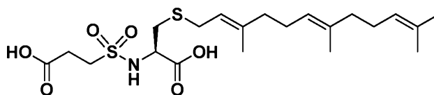
Compound N-80
