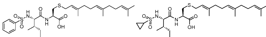
N-68;
