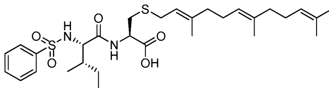
Compound N-68
