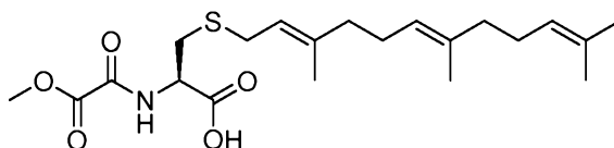
Compound N-10
