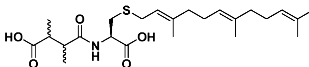
Compound N-30
