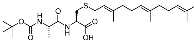
Compound N-3
