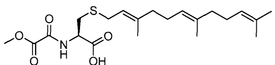
N-10;
