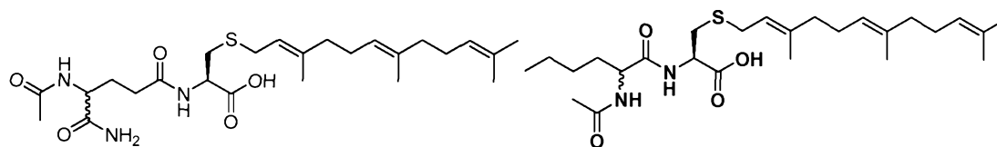
N-88;
