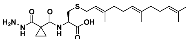
Compound N-75
