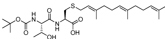
Compound N-56
