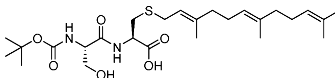
Compound N-55
