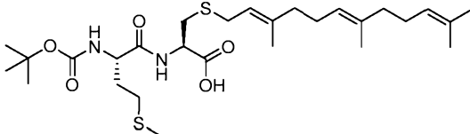
N-57;
