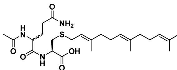
Compound N-61
