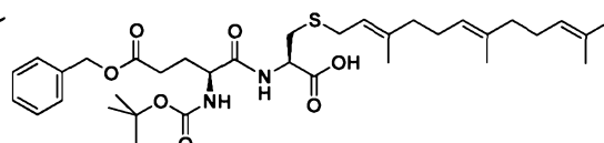
N-63;
