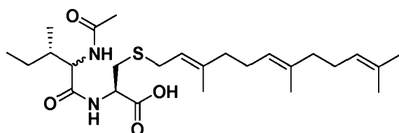
N-62;
