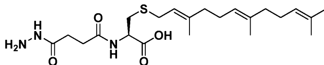
Compound N-76
