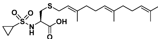
Compound N-79
