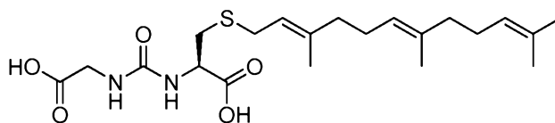
Compound N-15
