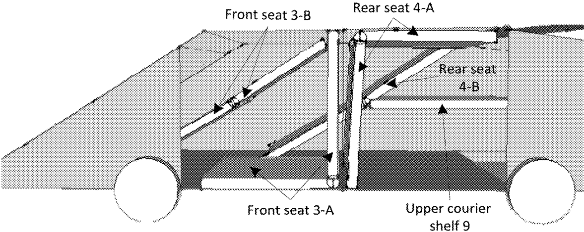
Configurable car 1 in dual seat mode
