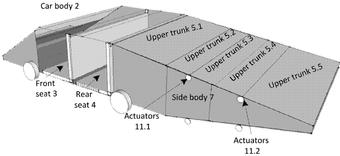
Configurable car 1 in passenger driving mode 7A
