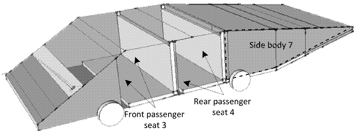
Configurable car 1 in passenger driving mode
