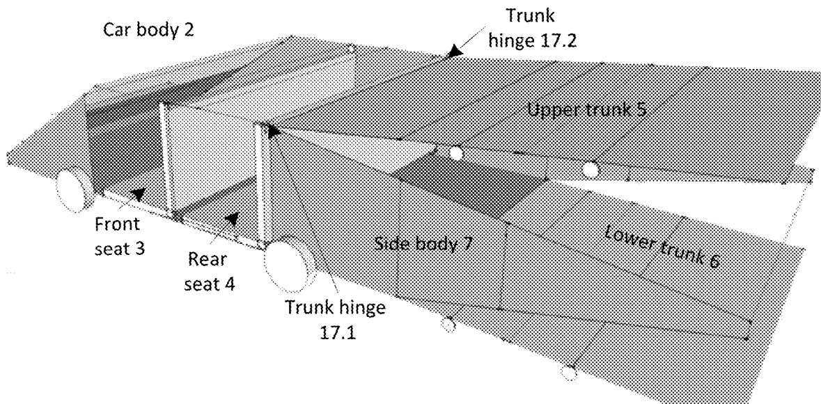
Configurable car 1 in loading mode 7B
