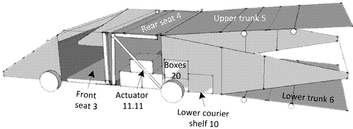
Configurable car 1 in courier loading mode 11A
