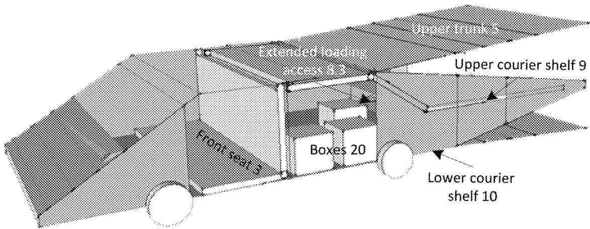
Configurable car 1 in courier loading mode
