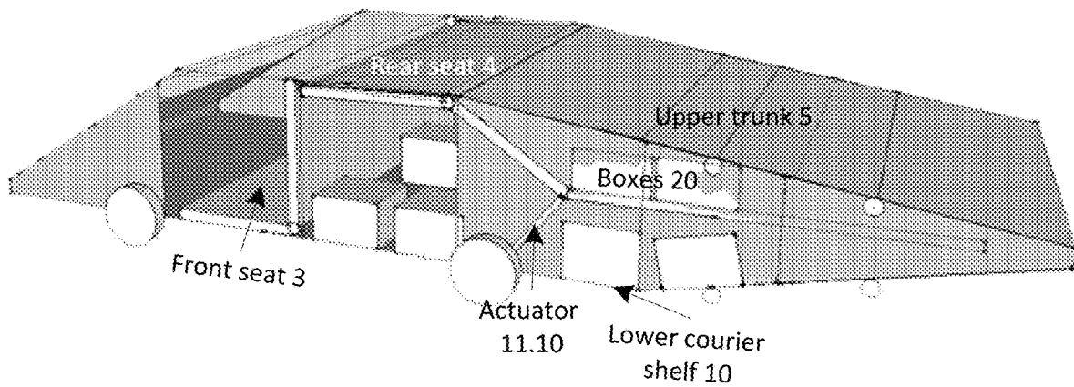
Configurable car 1 in courier driving mode
