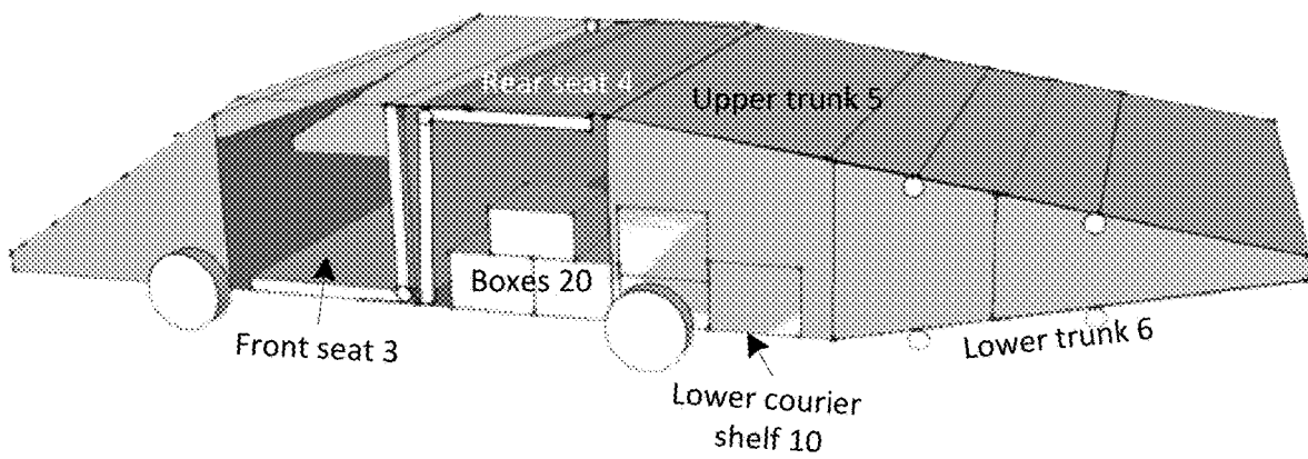
Configurable car 1 in courier driving mode 11B
