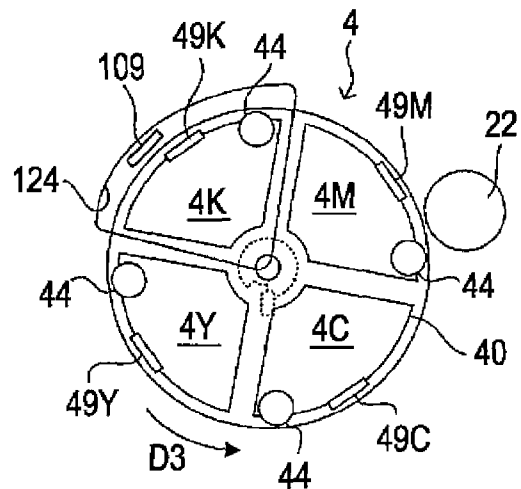
FIG. 3C DETACHMENT POSITION
