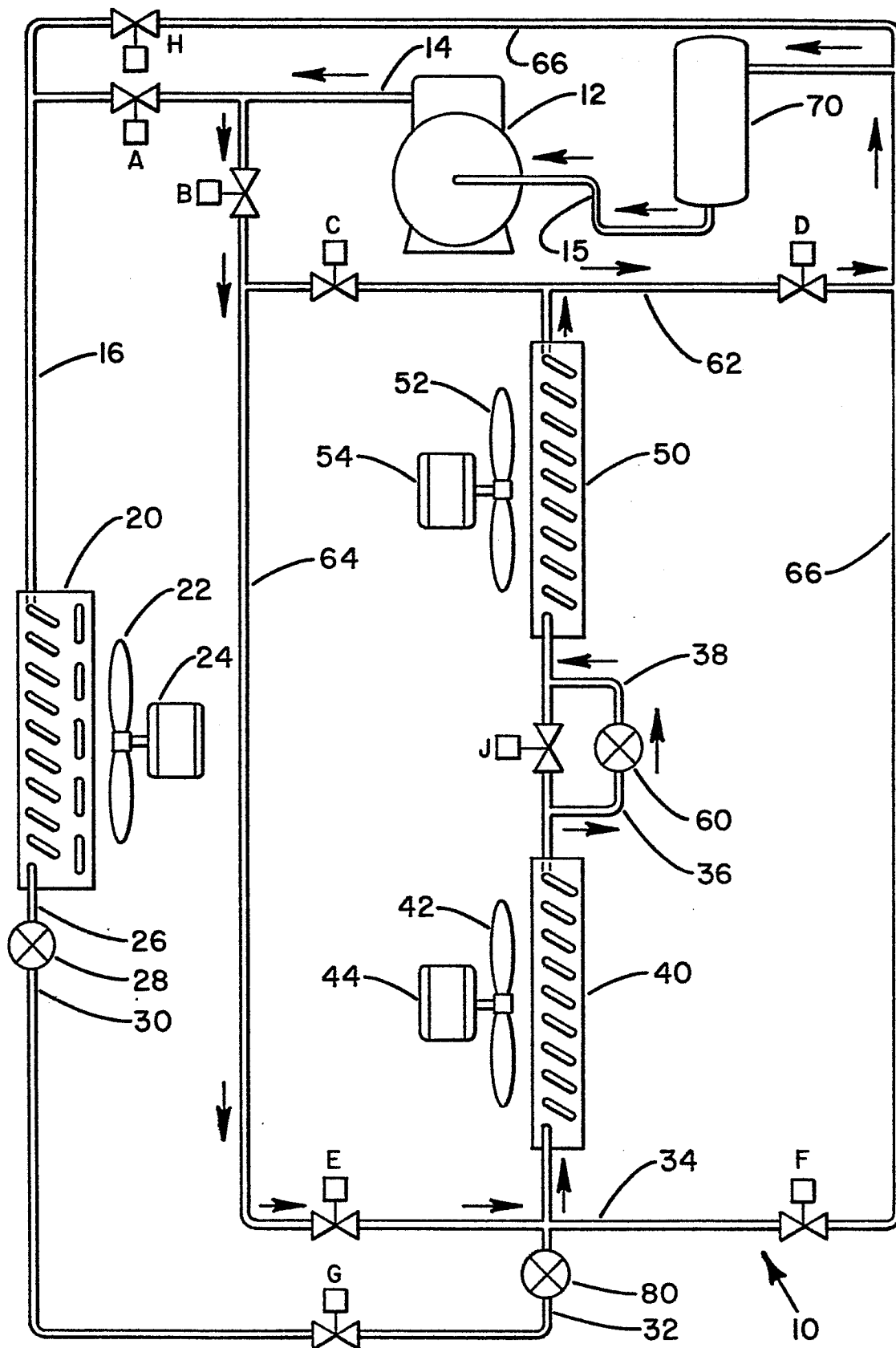
DEFROST CYCLE FOR COIL 2
