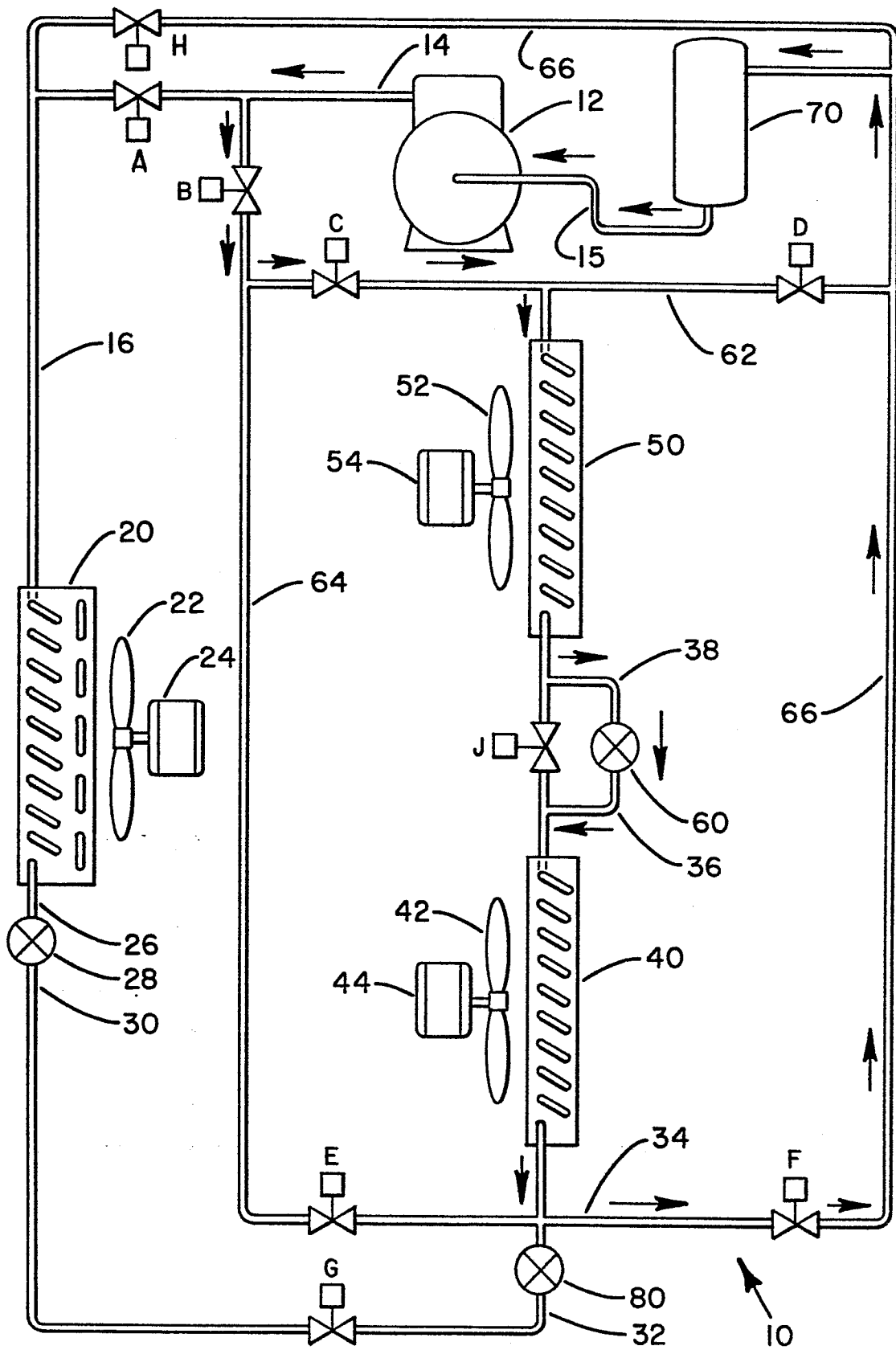
DEFROST CYCLE FOR COIL 1
