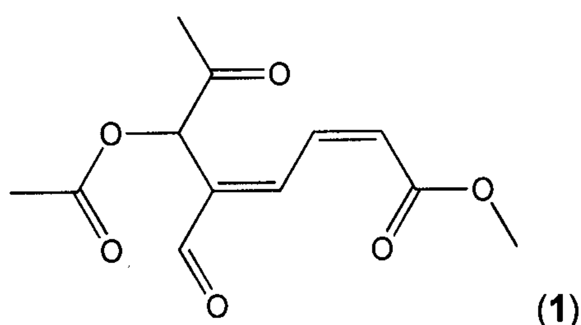
(2Z,4E)-methyl 6-acetoxy-5-formyl-7-oxoocta-2,4-dienoate
