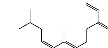
(6E, 8Z)-7,11-dimethyl-3-methylenedodeca-1,6,8-triene
