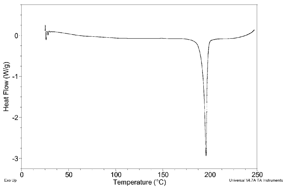
Figure 2: DSC Thermogram Form A
