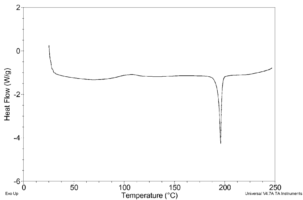
Figure 6: DSC Thermogram Form I
