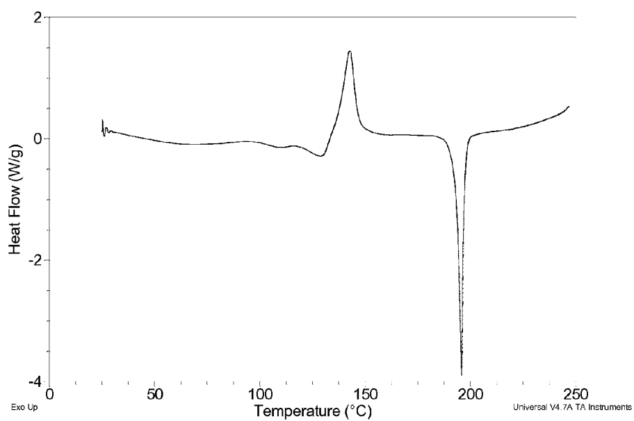
Figure 8: DSC Thermogram Form J
