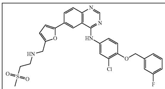
lapatinib
