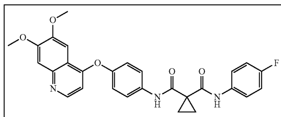
cabozantinib
