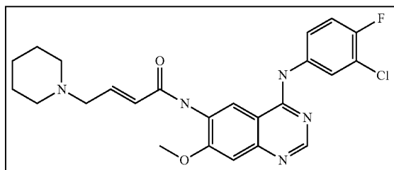
dacomitinib
