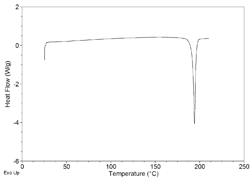
Figure 12: DSC Thermogram Succinate salt Form A 8
