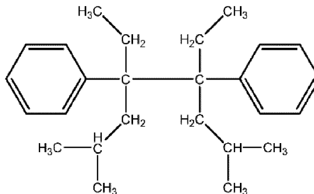
2,7-Dimethyl-4,5-diethyl-4,5-diphenyloctan (DBuDPH) (Struktur V)
