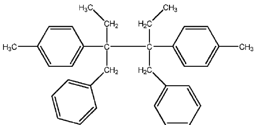
3,4-dibenzyl-3,4-ditolyl hexane (DBnDTH) (Structure VI)
