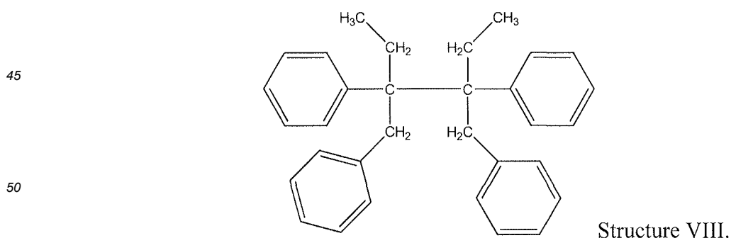
and, 3,4-dibenzyl-3,4-diphenyl hexane (Structure VIII)
