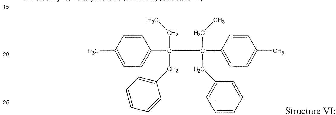
3,4-dibenzyl-3,4-ditolyl hexane (DBnDTH) (Structure VI)
