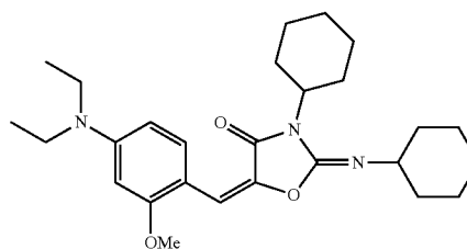
Sensitizing dye (4)
