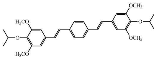
Sensitizing dye (3)
