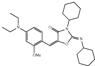
Compound SH-1
