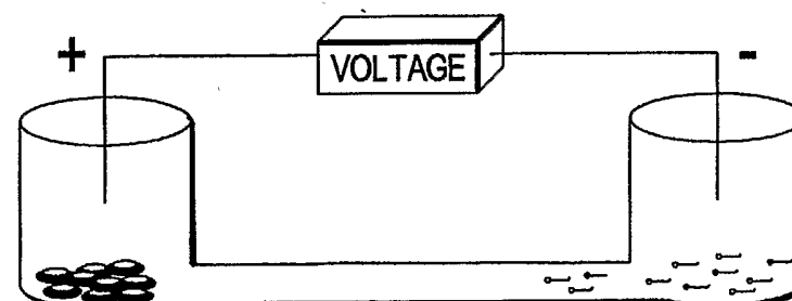
EVENTUALLY, SPERM CELLS ARE CONCENTRATED IN THE OUTLET WHILE THE EPITHELIAL CELLS ARE RETAINED IN THE INLET BY THE TENDENCY TO SETTLE, ADHERE AND THEIR ATTRACTION TO THE ANODE.
