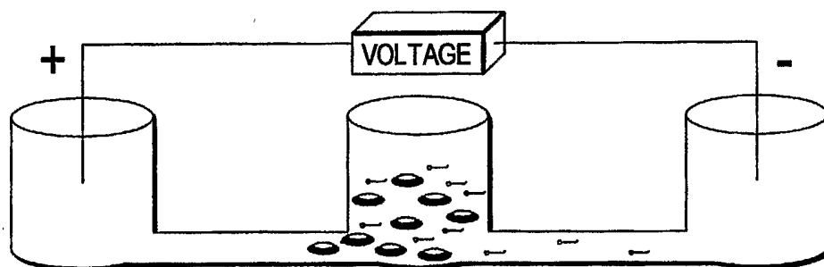
POTENTIAL APPLIED BETWEEN THE LEFT AND RIGHT RESERVOIRS. EPITHELIAL CELLS BEGIN TO SETTLE BASED ON THEIR SIZE AND DENSITY AS FLOW IS INITIATED BUT ARE ALSO ATTRACTED TO THE ANODE. EOF AND SPERM ELECTROPHORETIC MOBILITY IS TO THE CATHODE.
