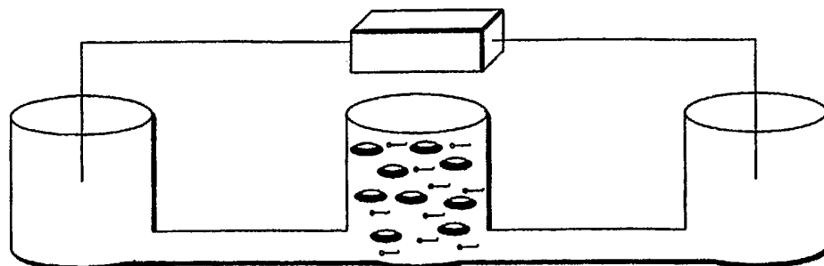
MIXTURE OF SPERM AND EPITHELIAL CELLS ADDED TO CENTRAL RESERVOIR.
