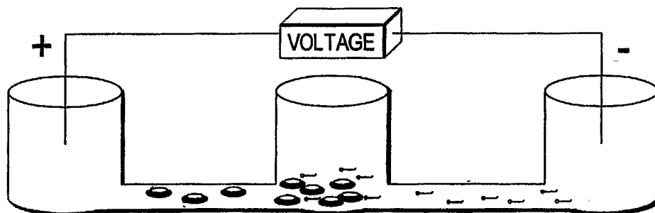
COMBINATION OF EOF AND DIFFERENTIAL ELECTROPHORETIC MOBILITY IN THE 3-CHAMBER SYSTEM SEPARATE CELLS.
