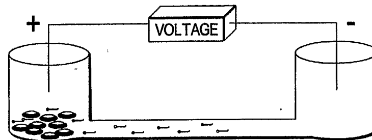
EPITHELIAL CELLS REMAIN IN THE INLET WHILE SPERM CELLS MIGRATE TOWARD THE OUTLET.
