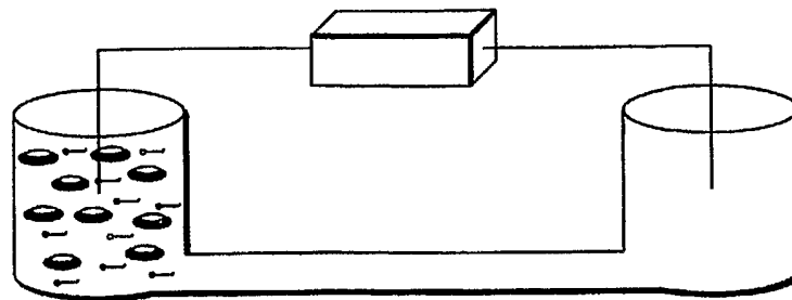
MIXTURE OF SPERM AND EPITHELIAL CELLS ADDED TO INLET RESERVOIR.
