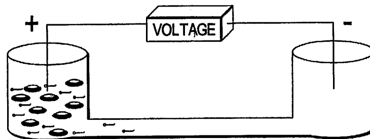
EPITHELIAL CELLS BEGIN TO SETTLE BASED ON THEIR SIZE AND DENSITY AS FLOW IS INITIATED (BY APPLYING VOLTAGE) BUT IN ADDITION TO THIS, THEIR ELECTROPHORETIC MOBILITY KEEPS THEM IN THE INLET RESERVOIR. IN CONTRAST, SPERM MIGRATE TOWARD THE CATHODE BASED ON BOTH THEIR ELECTROPHORETIC MOBILITY AND ON THEIR MIGRATION WITH THE EOF.
