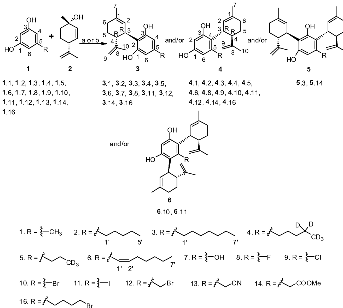
Scheme 7
