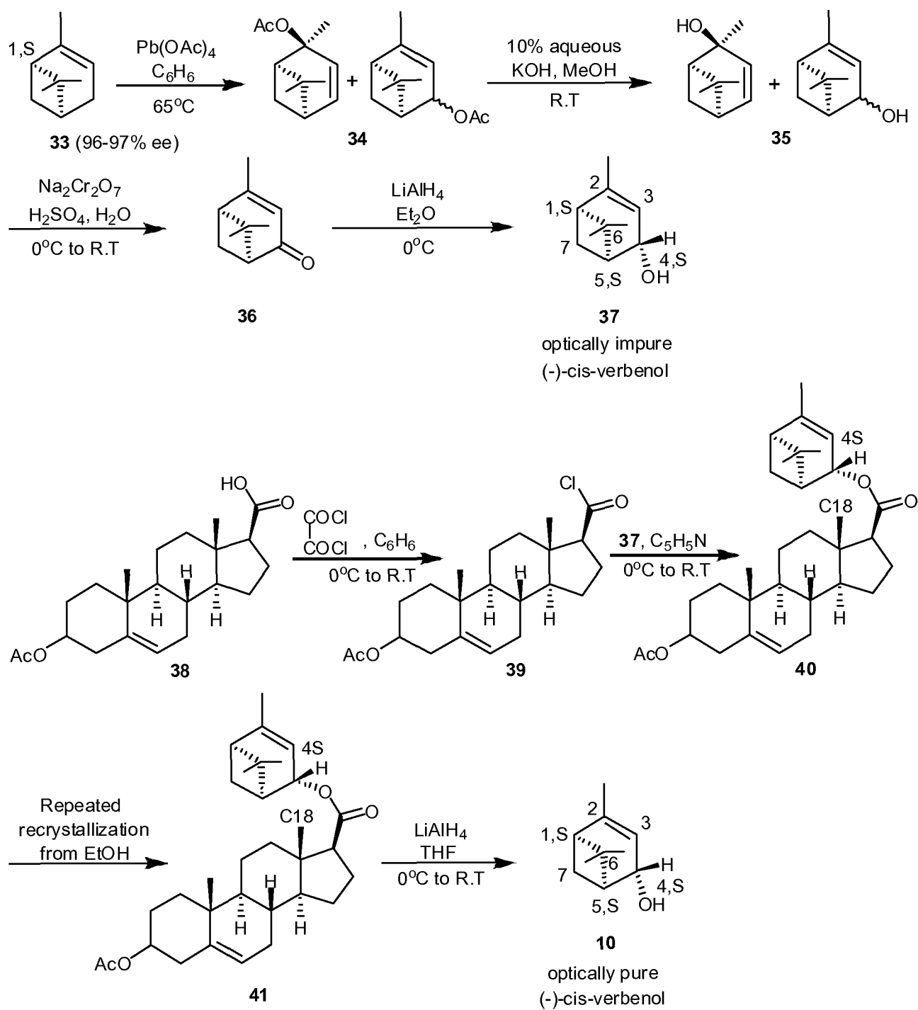
Scheme 6
