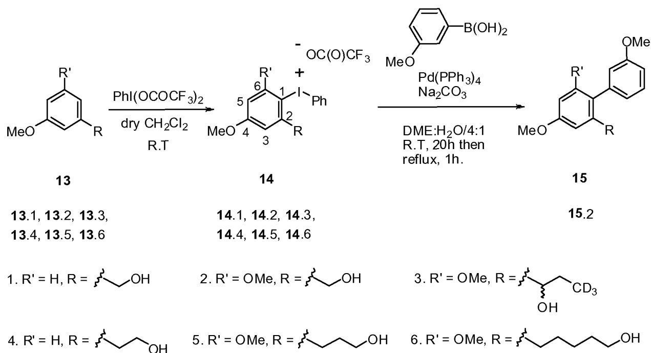
Scheme 10
