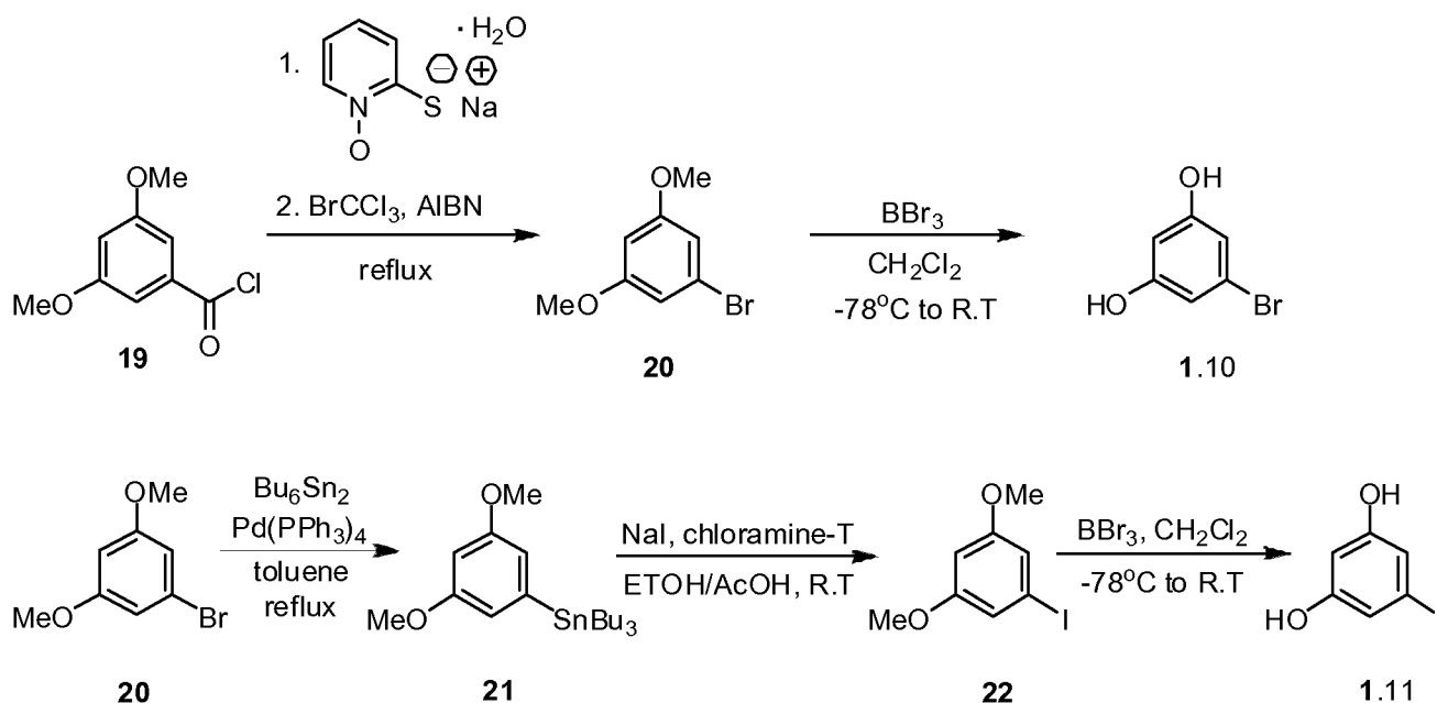
Scheme 3
