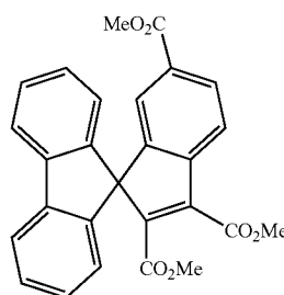
Spirodihydroindolizines
