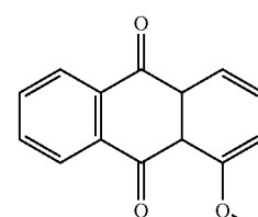
Quinone
