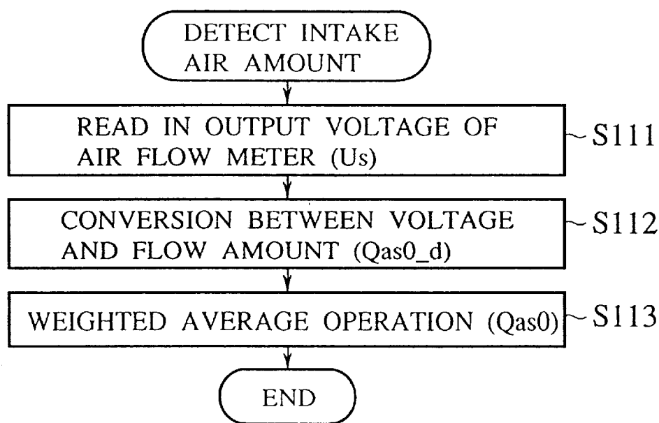
INTAKE AIR AMOUNT DETECTING FLOW CHART
