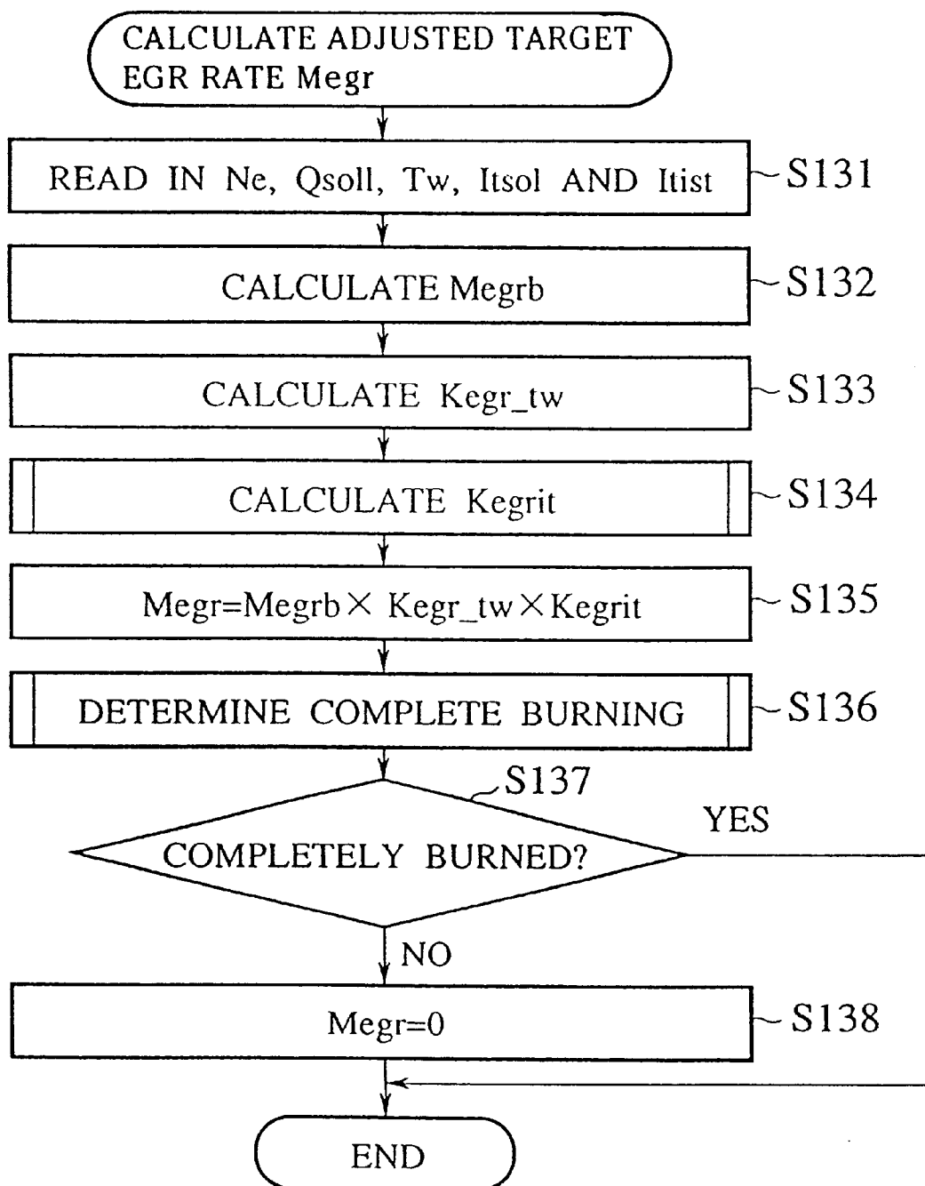
TARGET EGR RATE CALCULATING FLOW CHART
