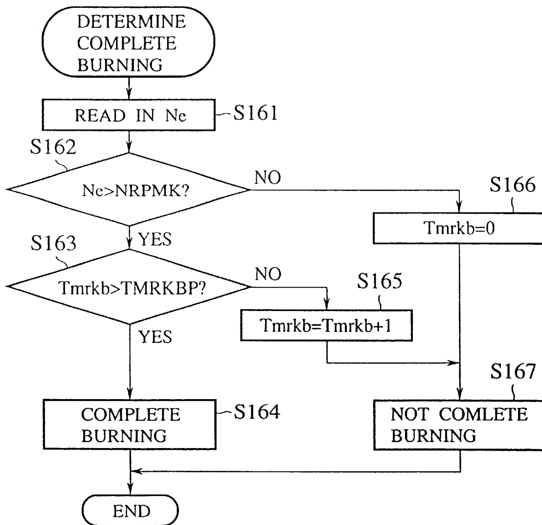
COMPLETE BURNING DETERMINATION FLOW CHART
