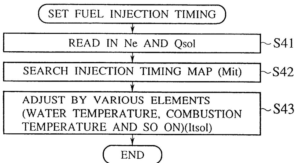
TARGET INJECTION TIMING SETTING FLOW CHART
