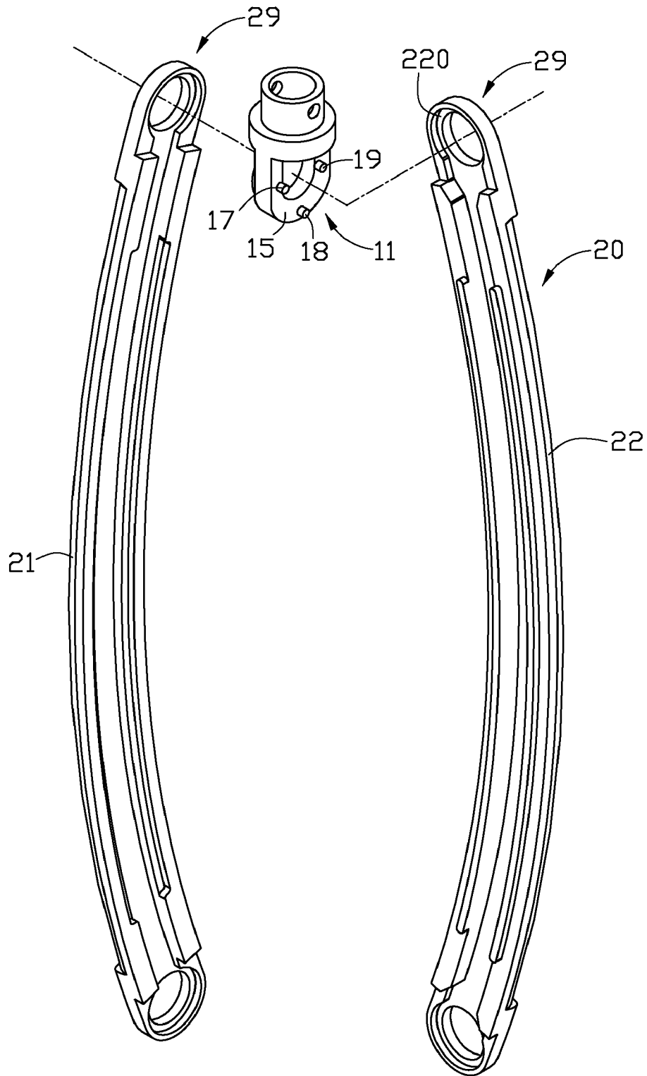
FIG. 4 (RELATED ART)
