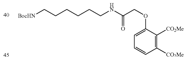
(2) Synthesis of dimethyl 3-((2-((6-((tert-butoxycarbonyl)amino)hexyl)amino)-2-oxoethoxy)phthalate
