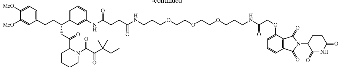
Scheme for Synthesis of Amino Acid-Thalidomide Linker
