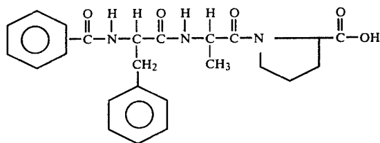
Benzoylphenylalanylalanylproline
