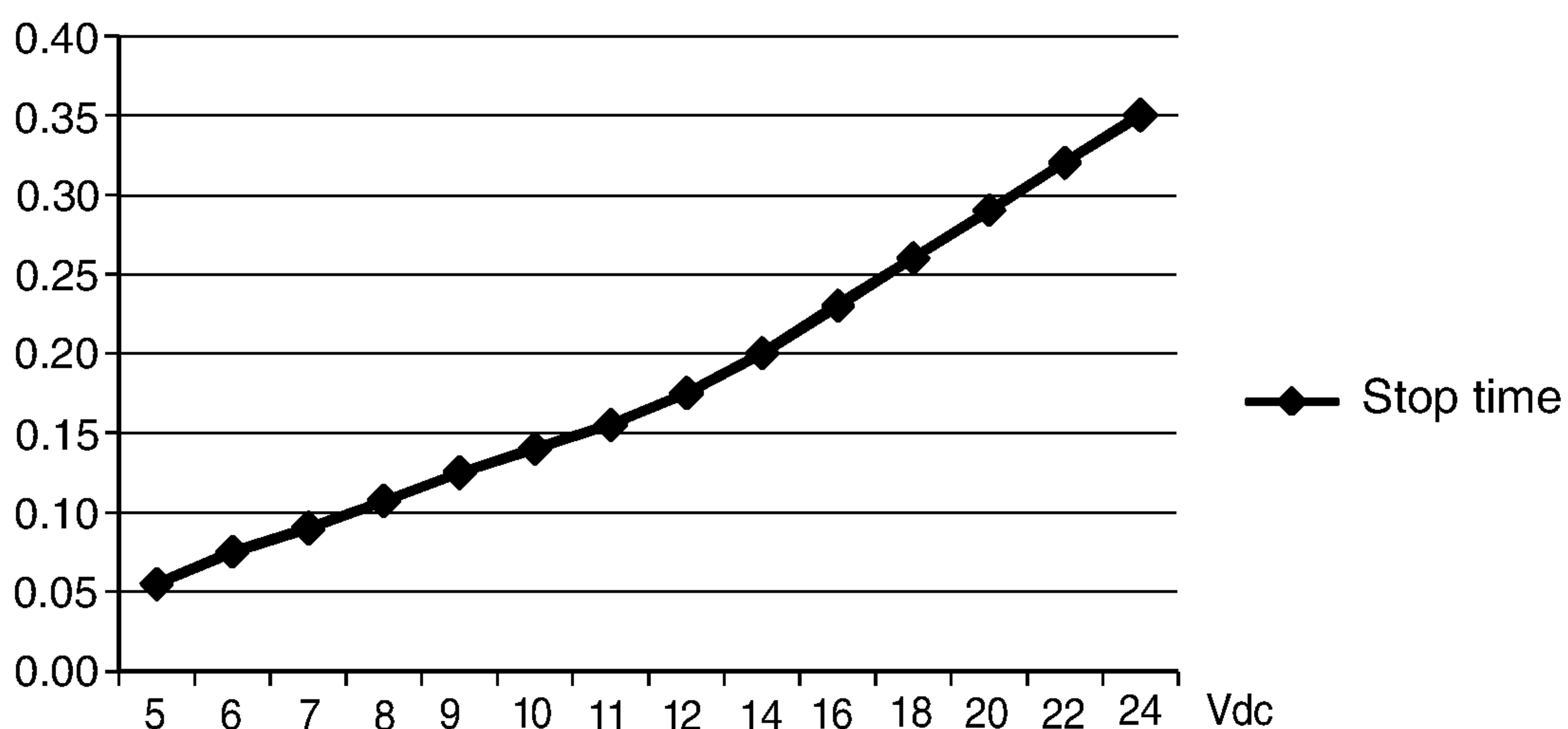
Pump rotations to standstill
