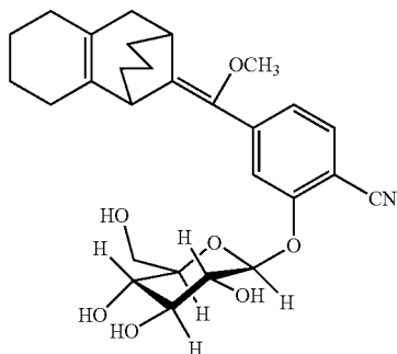
Synthesis of [(4-methoxy-4-(3-β-D-glucoside-4-cyanophenyl)methoxymethylene tricyclo[7.3.1.0 2,7 ]tridec-2,7-enein
