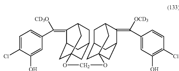
(c). Synthesis of bis-[(3-phosphoryloxy-4-chlorophenyl)methoxy(D3)methylene-5-oxy-adamantane, disodium salt]methane
