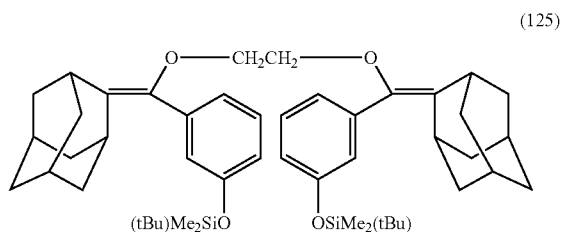
(f). Synthesis of bis[(3-hydroxyphenyl)methylenoxymethylene adamantane]
