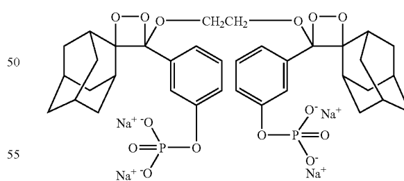
(g). Synthesis of bis[(3-phosphoryloxyphenyl)methylenoxymethylene adamantane, disodium salt]
