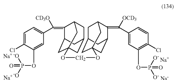
Photooxidation of bis-[(3-phosphoryloxy-4-chlorophenyl)methoxy(D3)methylene-5-oxy-adamantane, disodium salt]methane
