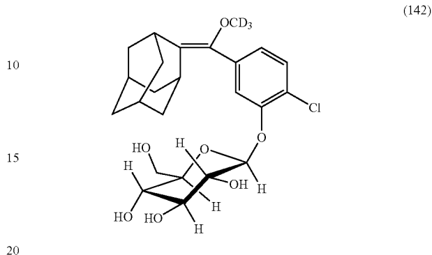
Synthesis of [(4-Methoxy(D 3 )-4-(3-β-D-glucoside-4-chlorophenyl)]spiro[1,2-dioxetane-3,2'-adamantane]
