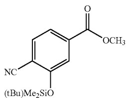
(c). Synthesis of (3-silyloxyoxy-4-cyanophenyl)methoxymethylene tricyclo[7.3.1.0 2,7 ]tridec-2,7-ene
