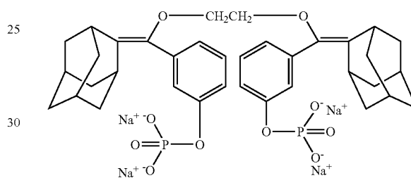
(h). Synthesis of Bis{[(4-methylenoxy)-4-(3-phosphoryloxyphenyl)]spiro[1,2-dioxetane-3,2'-adamantane], disodium salt} (146)
