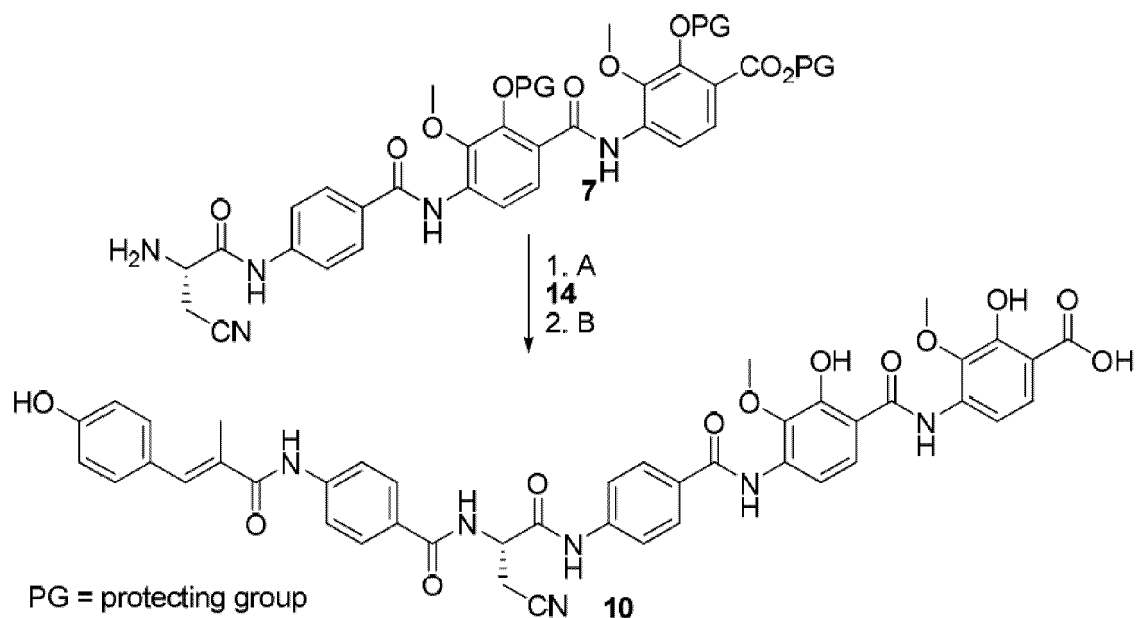
Scheme 23
