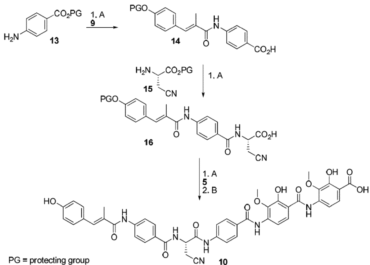
Scheme 23
