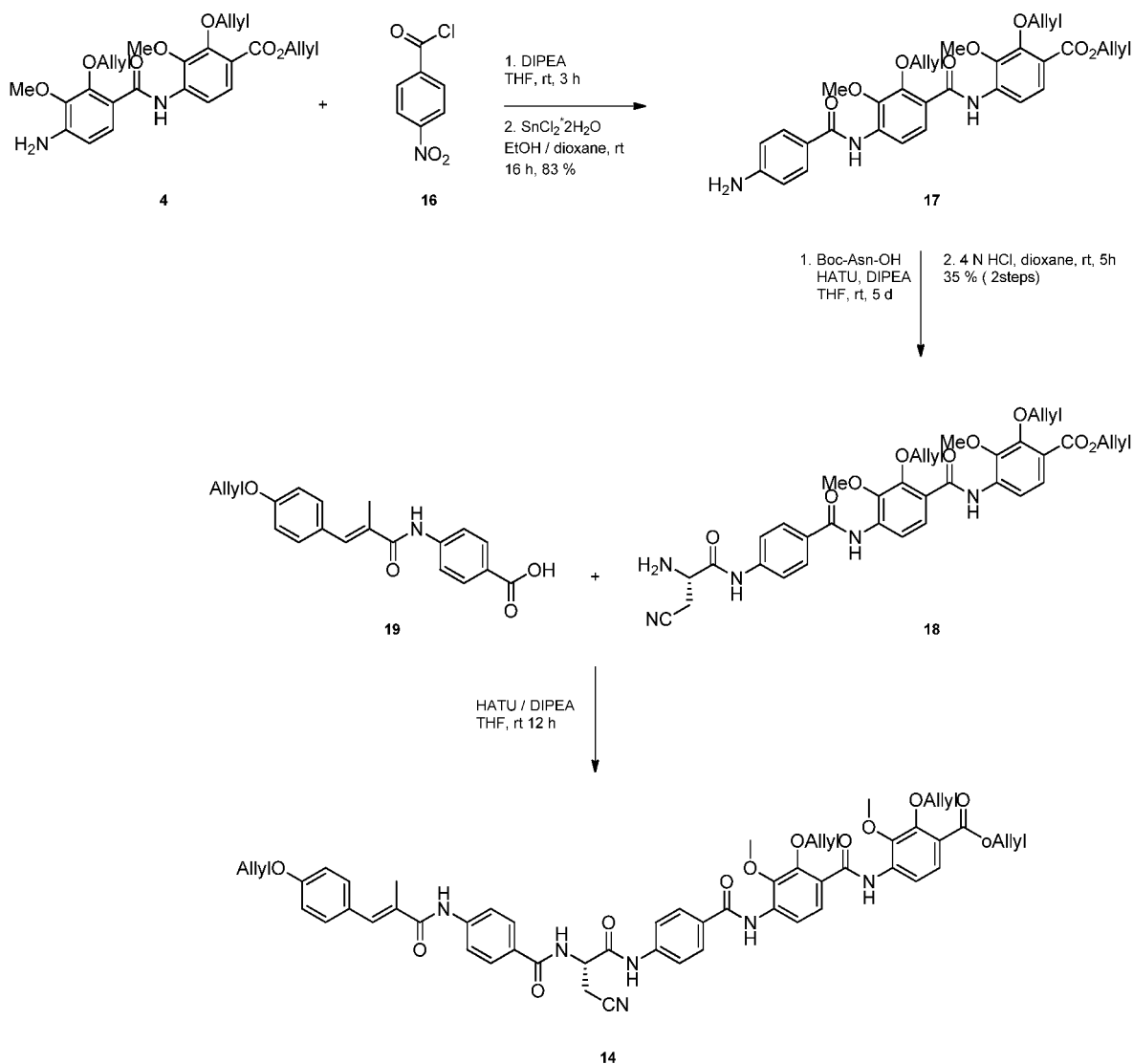
Scheme 17
