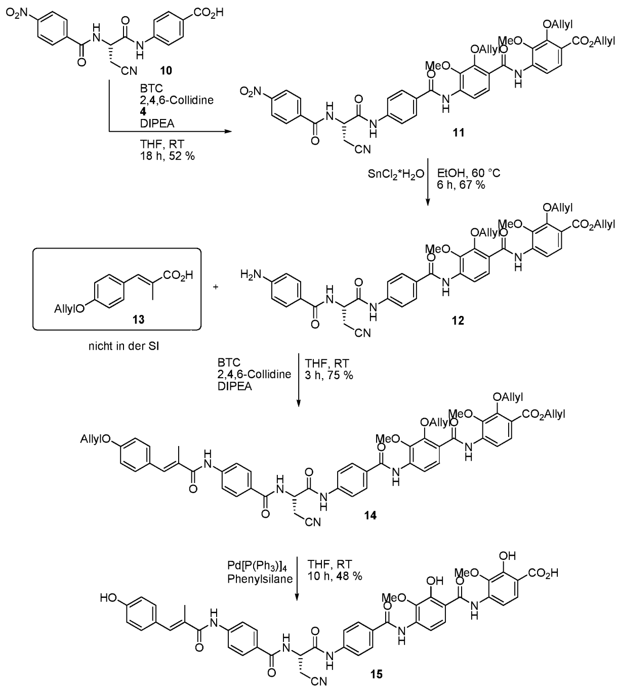
Scheme 16
