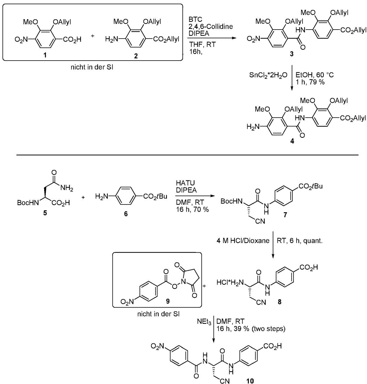
Scheme 15
