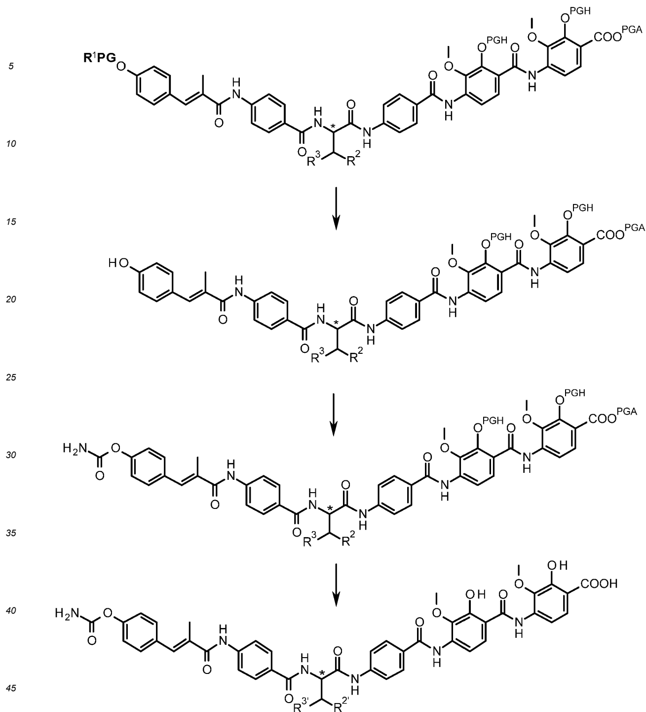
Scheme 18
