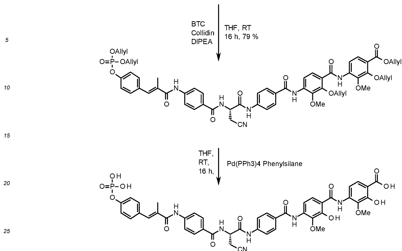
Scheme 13:
