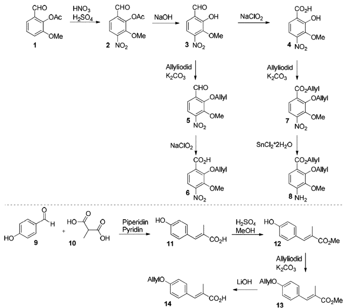
Scheme 19
