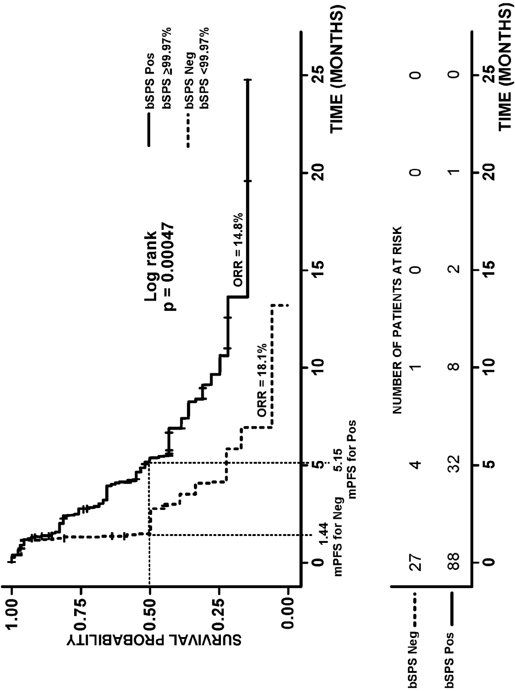
bystander_memb(meanOD)_binary_r50_cut25
