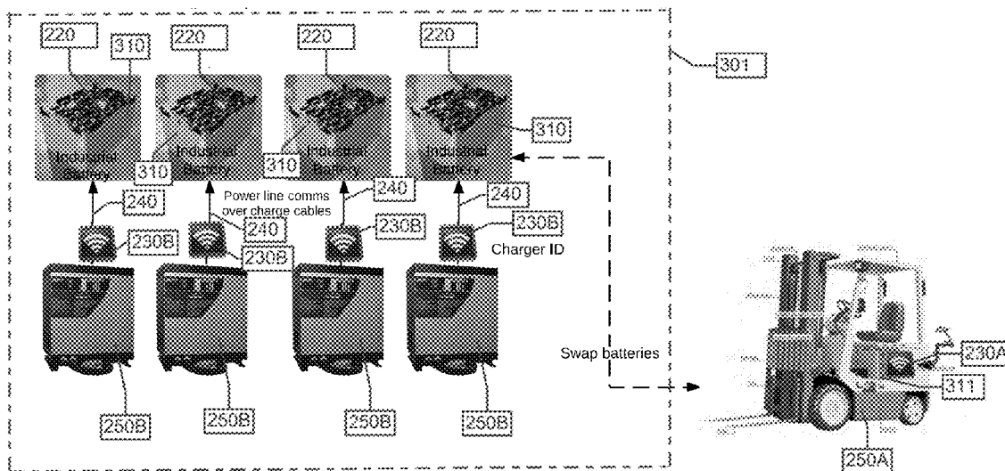
Battery selector System
