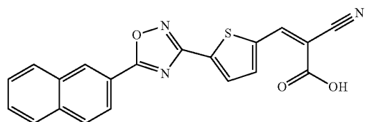
(Z)-2-cyano-3-(5-(5-(naphthalen-2-yl)-1,2,4-oxadiazol-3-yl)thiophen-2-yl)acrylic acid
