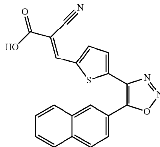
(E)-2-cyano-3-(5-(5-(naphthalen-2-yl)-1,2,3-oxadiazol-4-yl)thiophen-2-yl)cianoacrylic acid
