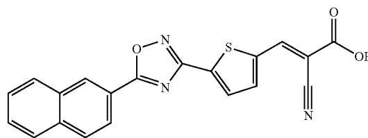
(E)-2-cyano-3-(5-(5-(naphthalen-2-yl)-1,2,4-oxadiazol-3-yl)thiophen-2-yl)cianoacrylic acid
