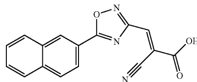
(E)-2-cyano-3-(5-(naphthalen-2-yl)-1,2,4-oxadiazol-3-yl)acrylic acid
