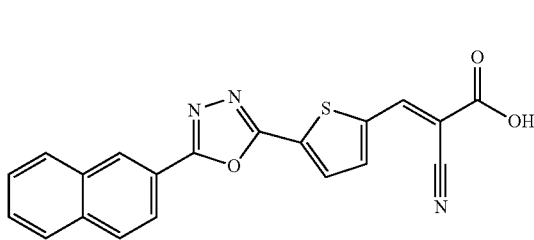
(E)-2-cyano-3-(5-(5-(naphthalen-2-yl)-1,3,4-oxadiazol-2-yl)thiophen-2-yl)cianoacrylic acid
