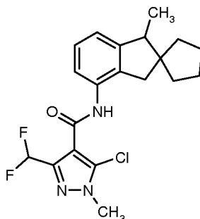
5-chloro-3-(difluoromethyl)-1-methyl-N-(1'-methyl-1',3'-dihydrospiro[cyclopentane-1,2'-inden]-4'-yl)-1H-pyrazole-4-carboxamide (example 33)
