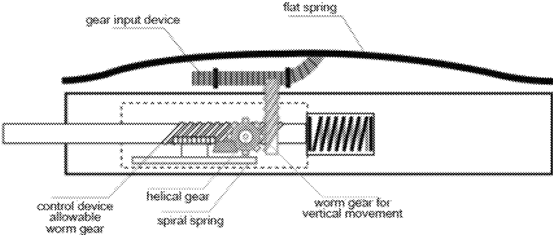
front view of gear box
