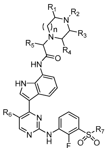
Formula (I)
