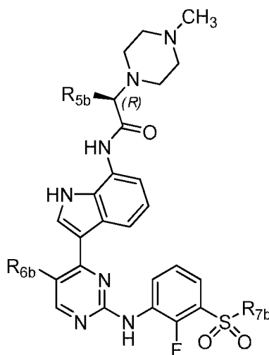
Formula (Ib)
