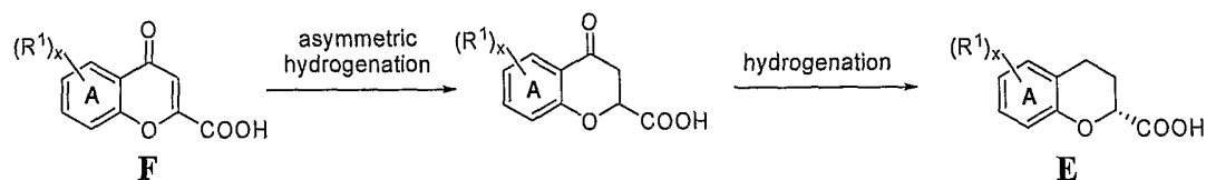
Scheme 17
