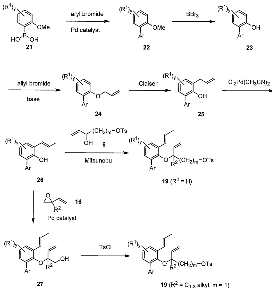
Scheme 7
