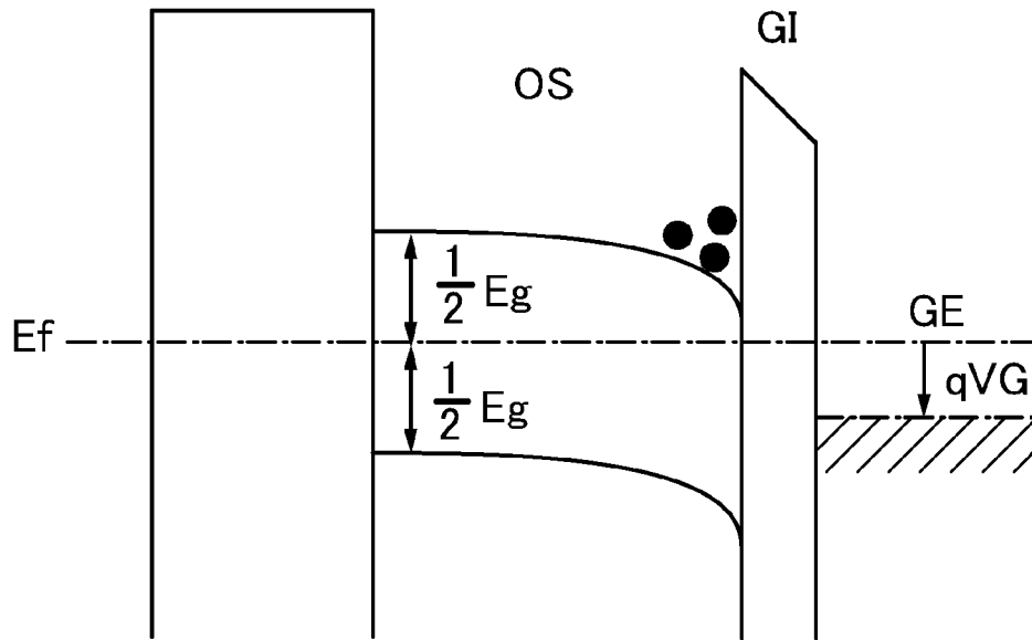
Energy band diagram of B-B' section ( V_G > 0 )
