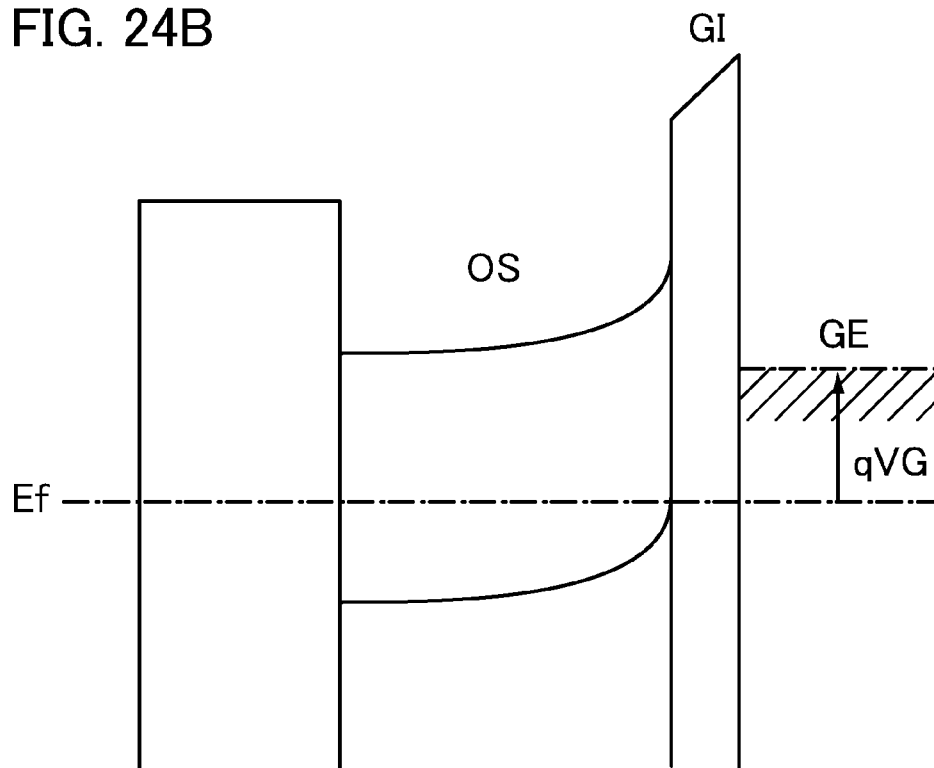
Energy band diagram of B-B' section ( V_G < 0 )
