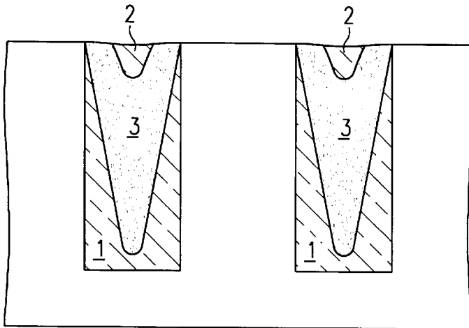
FIG. 3C SOG/LTO etchback
