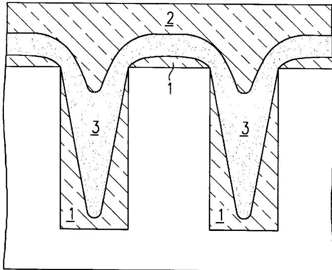
FIG. 3B LTO deposition and SOG-2 spin/cure
