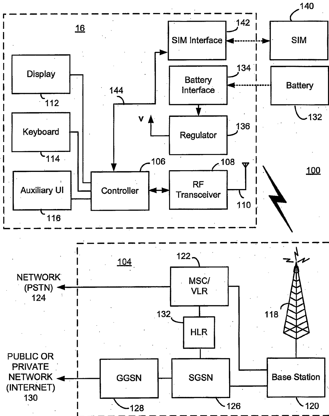
FIG. 5: GPRS Device
