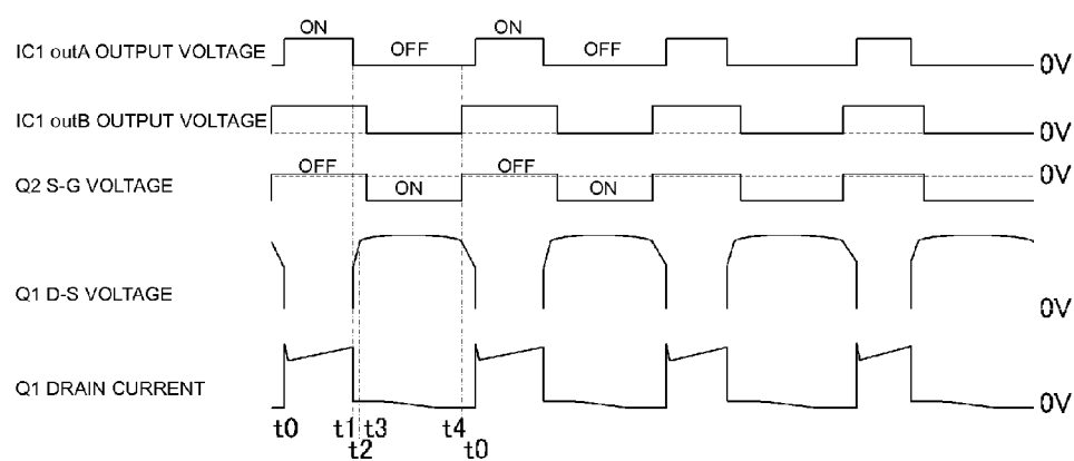
FIG. 2 PRIOR ART
